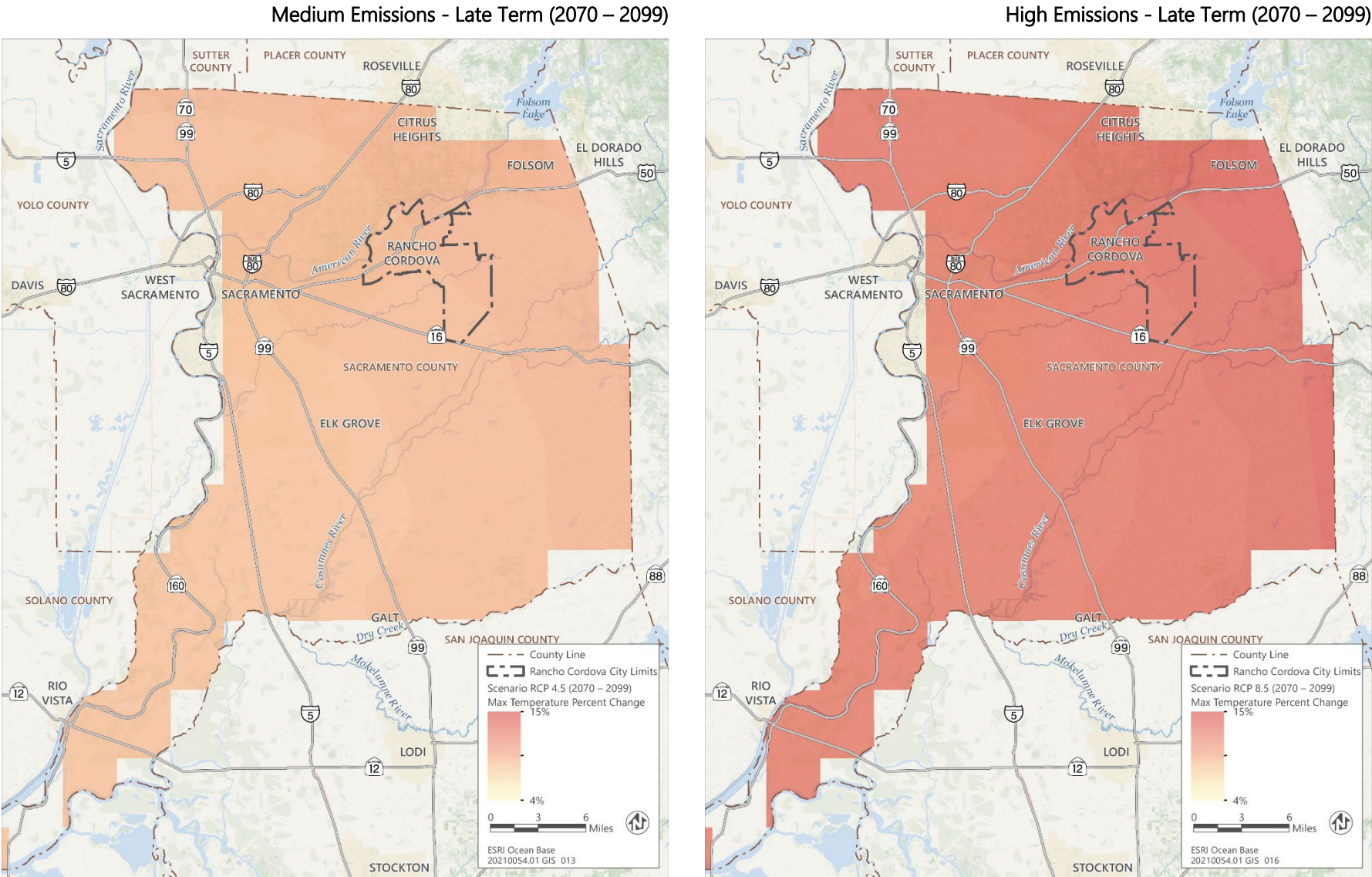
Figure 4 Sacramento County Annual Average Maximum Temperature through 2099
