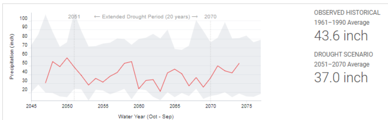
Figure 8 El Dorado County Long-Term Drought Scenario (2051-2070)
