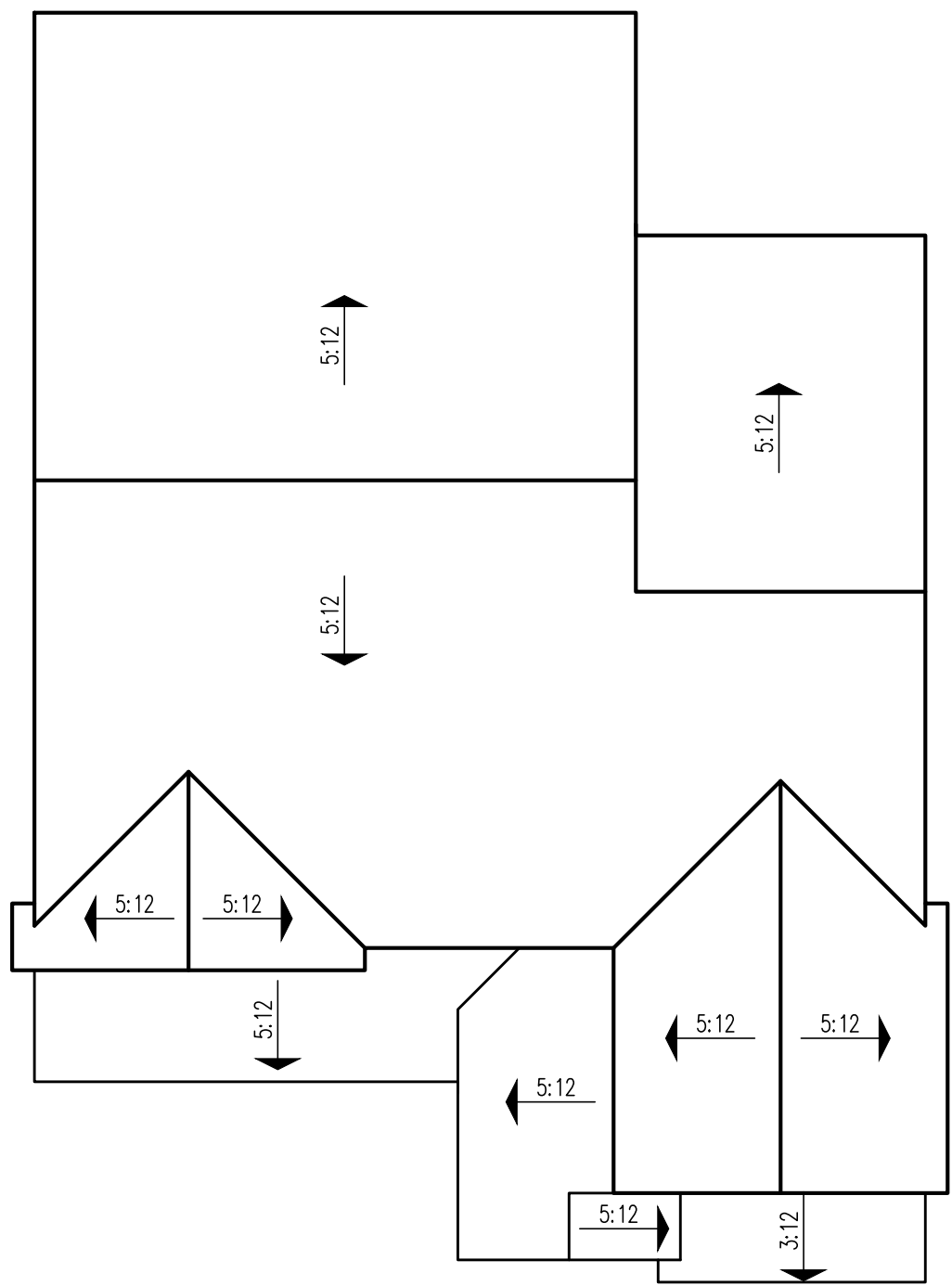
Roof Plan 'A' - Spanish Eclectic
