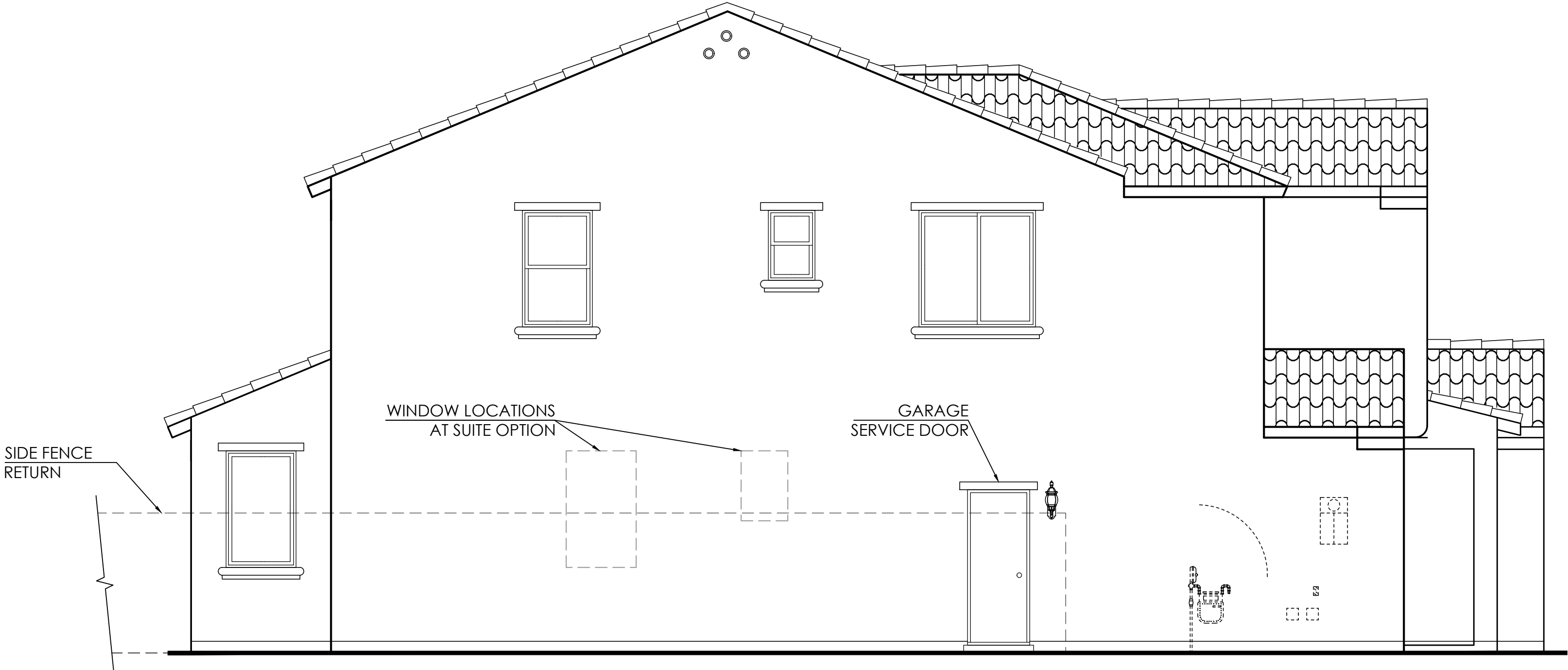
Left Elevation
