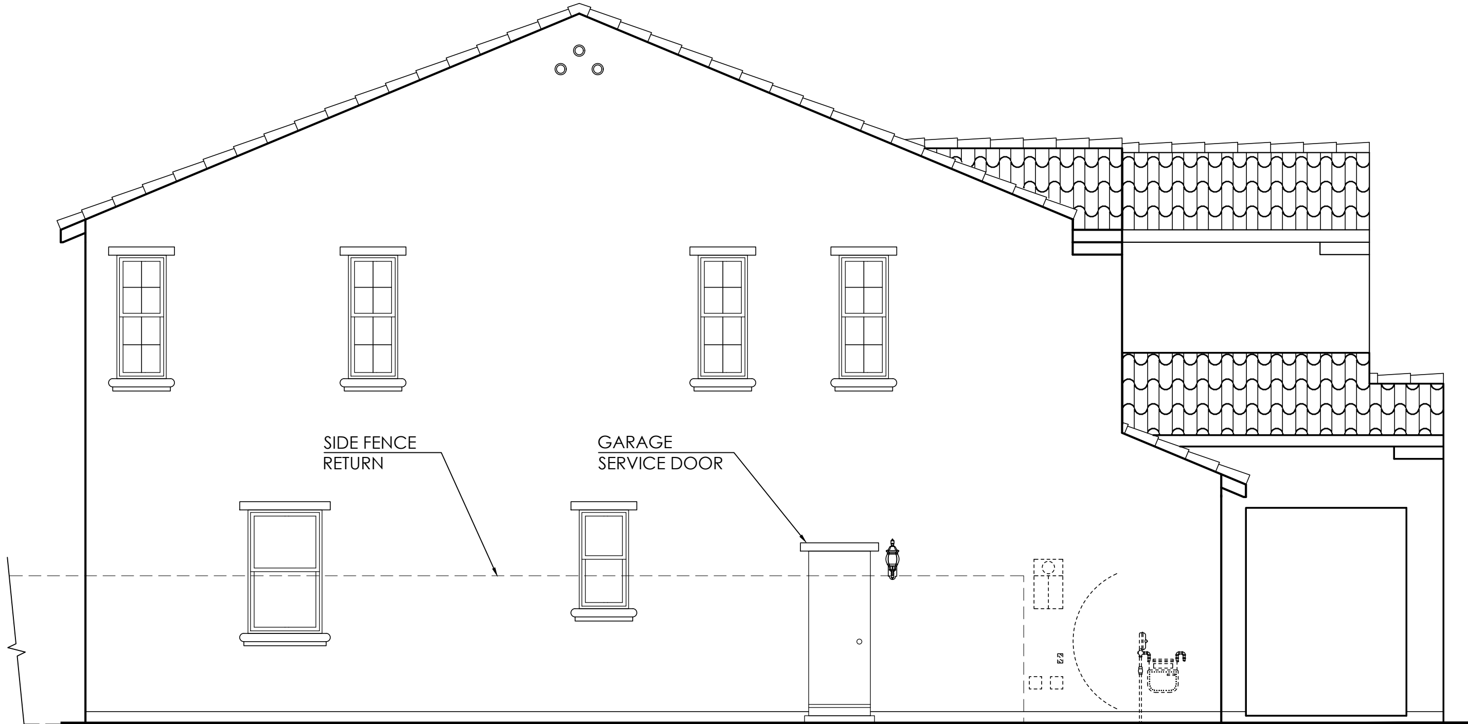
Left Elevation
