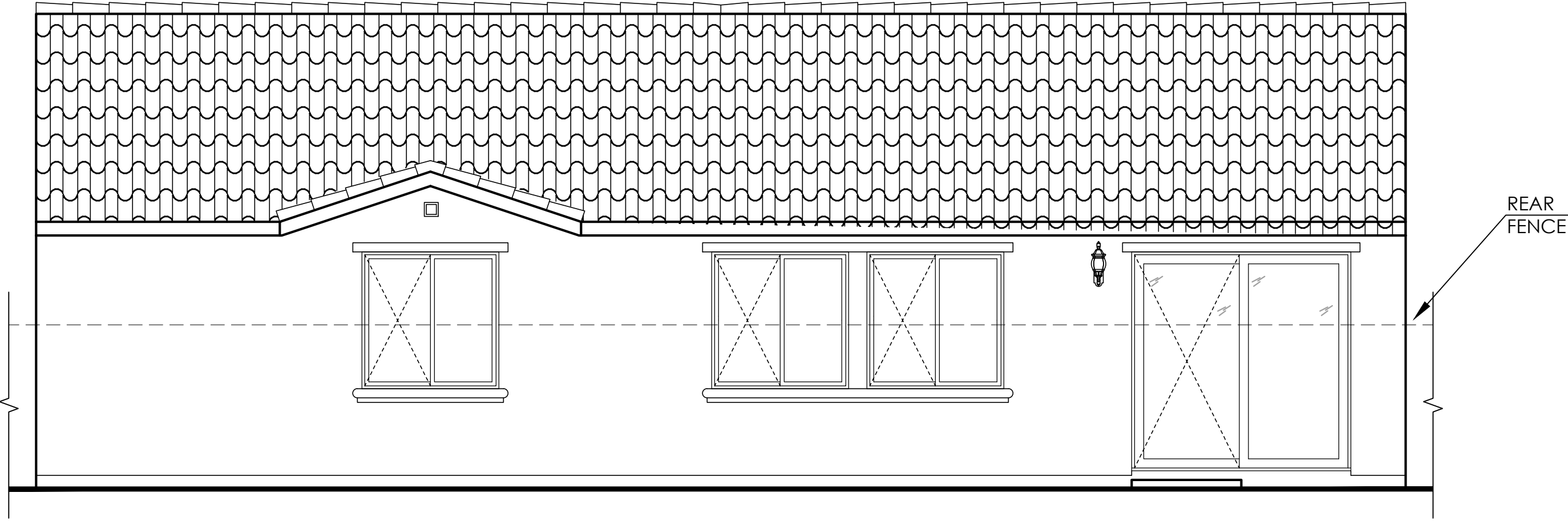
Rear Elevation
