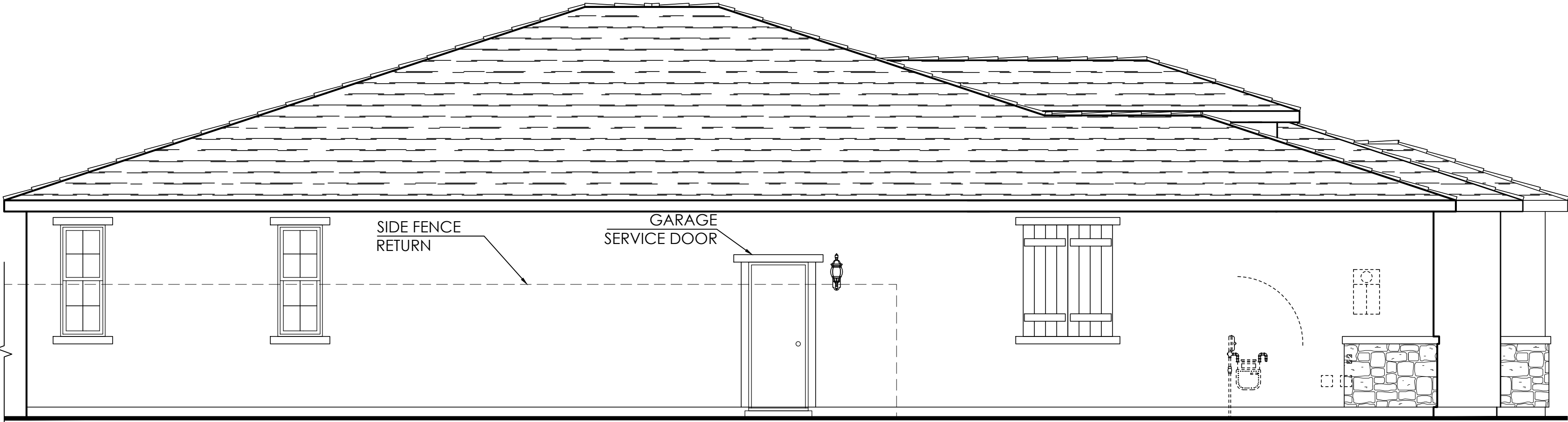
Left Elevation
