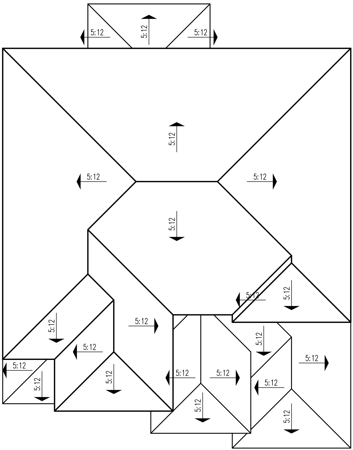
Roof Plan 'B' - Tuscan
