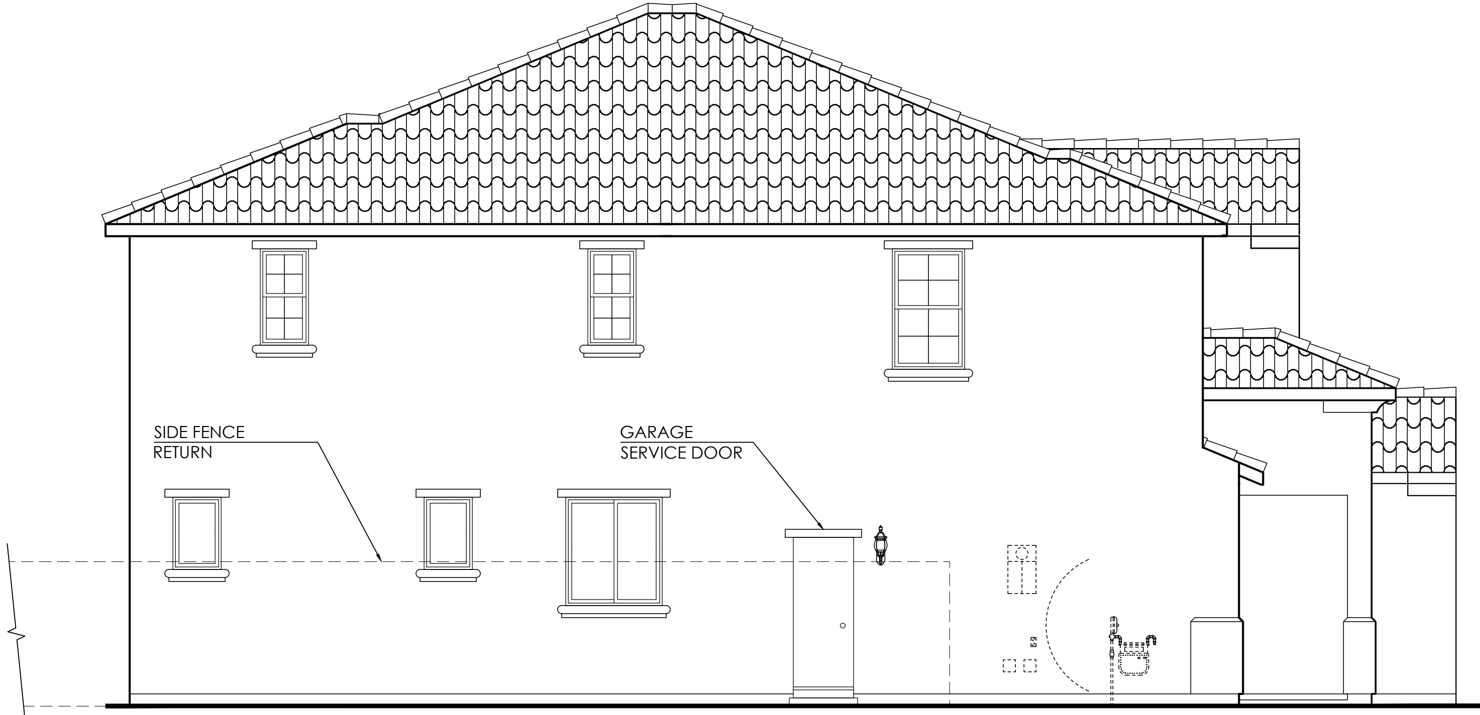
Left Elevation
