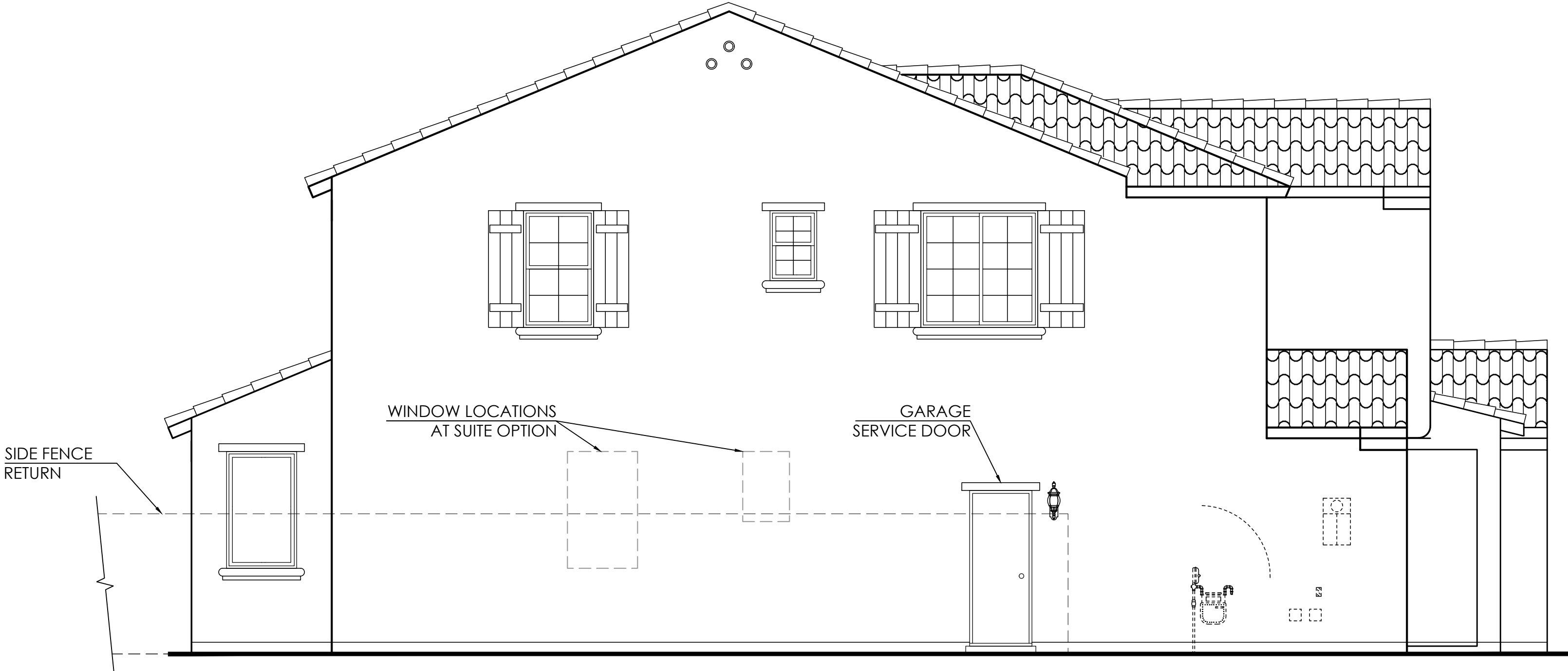
Left Elevation
