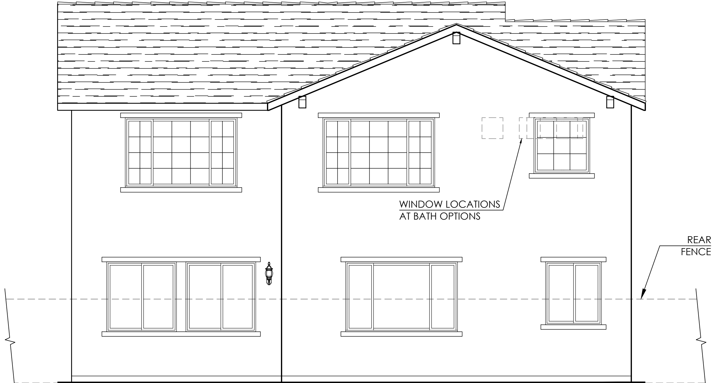
Rear Elevation
