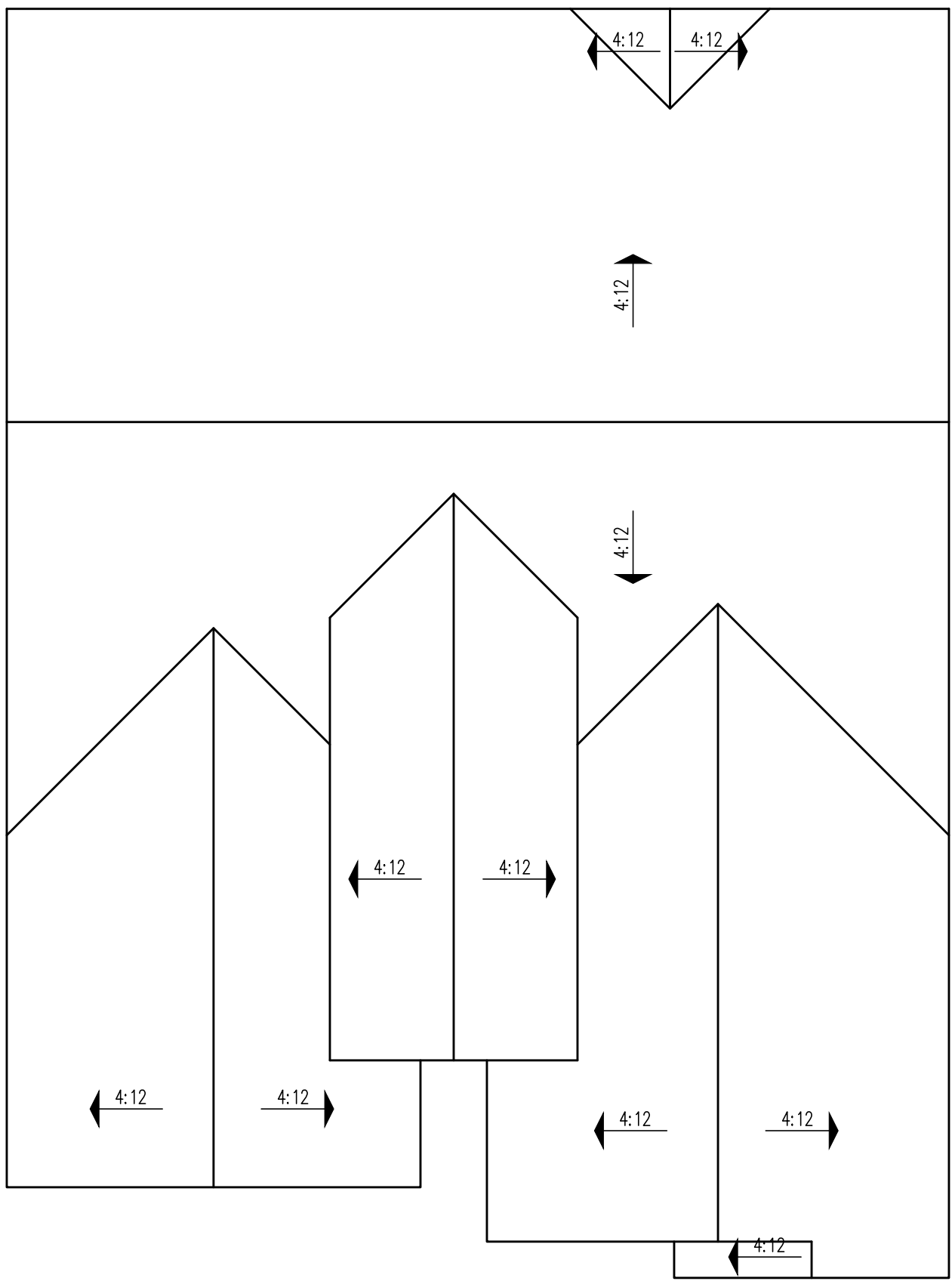
Roof Plan 'C' - Modern Farmhouse
