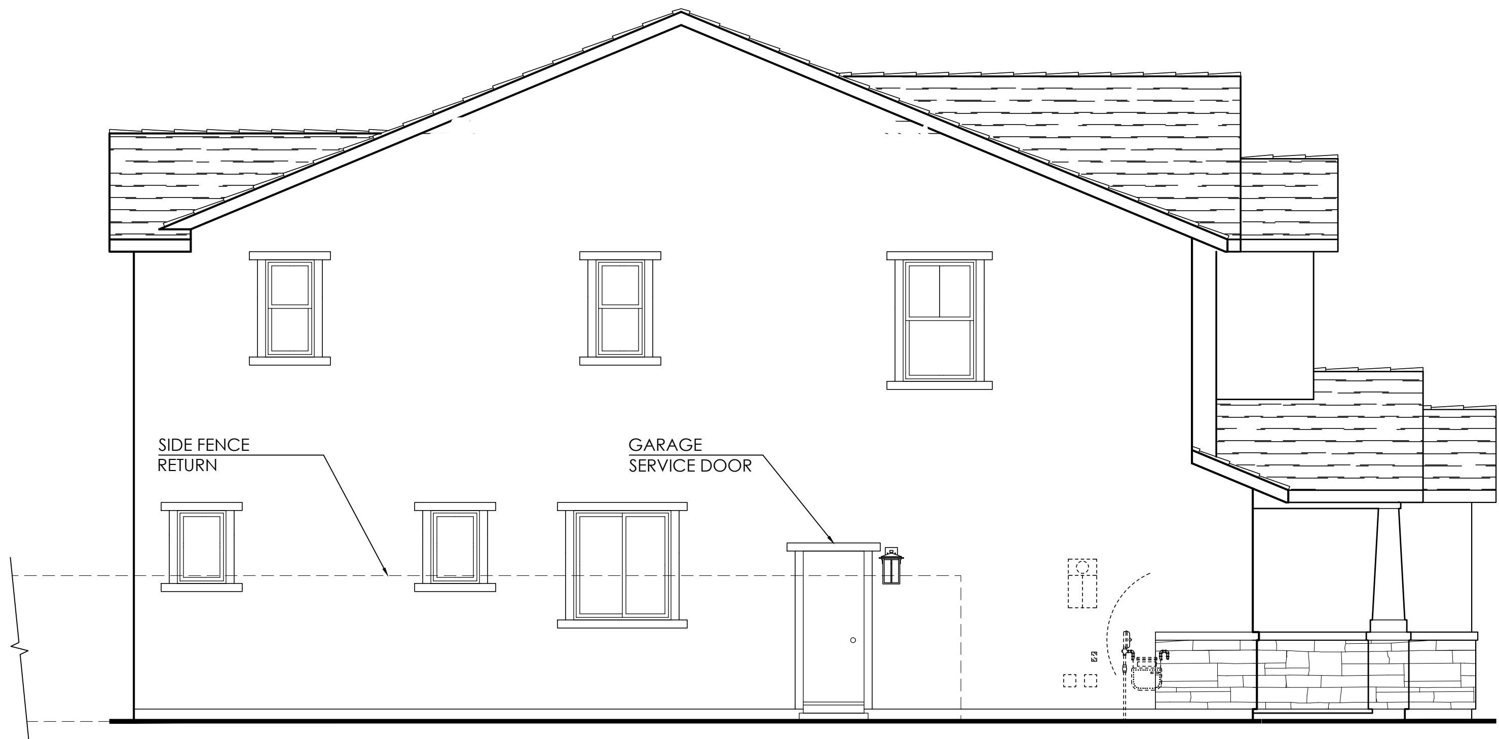
Left Elevation
