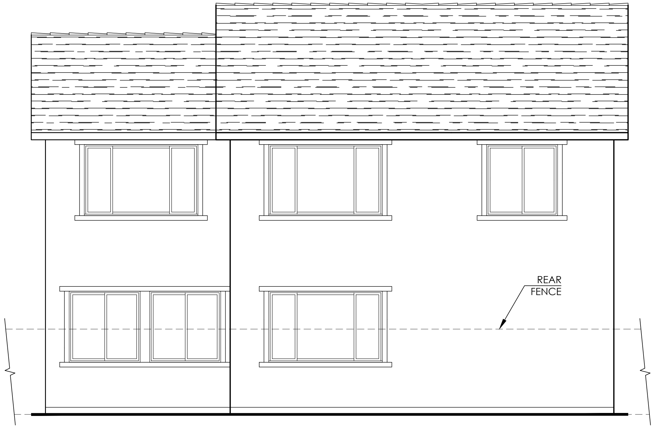
Rear Elevation
