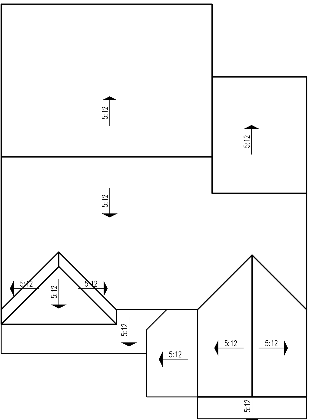
Roof Plan 'B' - Tuscan
