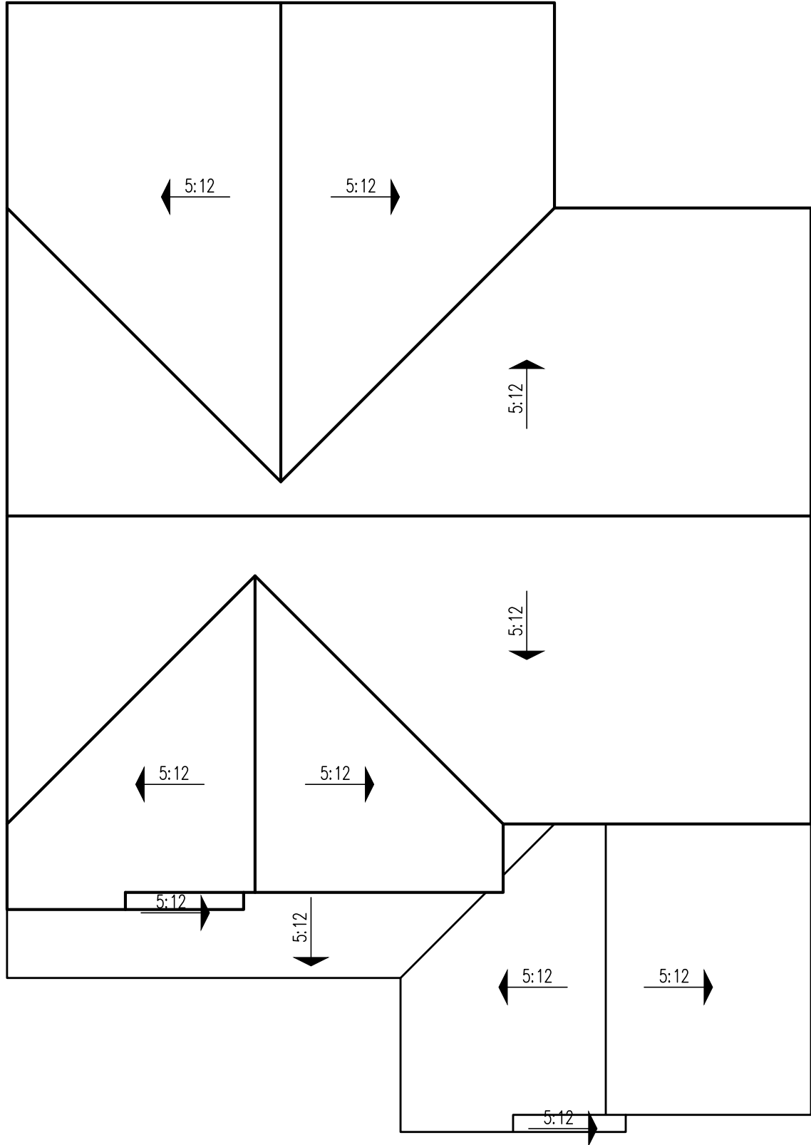
Roof Plan 'C' - Modern Farmhouse
