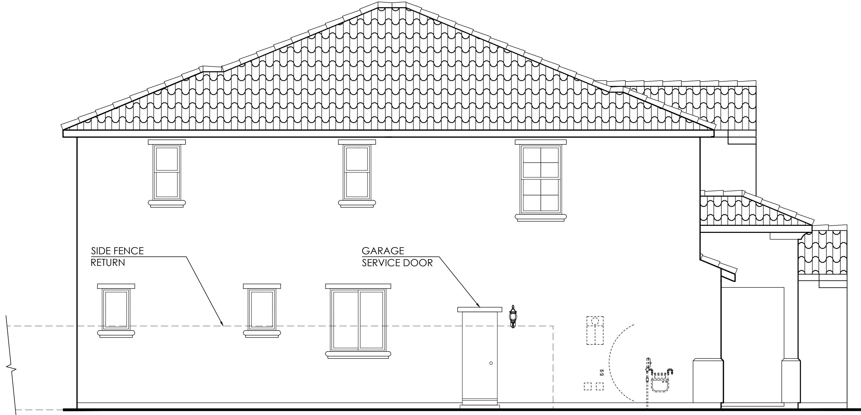
Left Elevation
