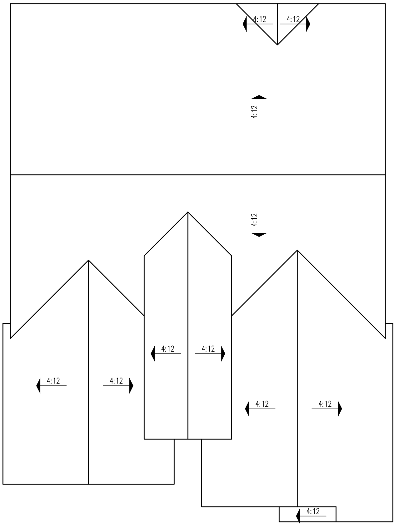
Roof Plan 'A' - Spanish Eclectic
