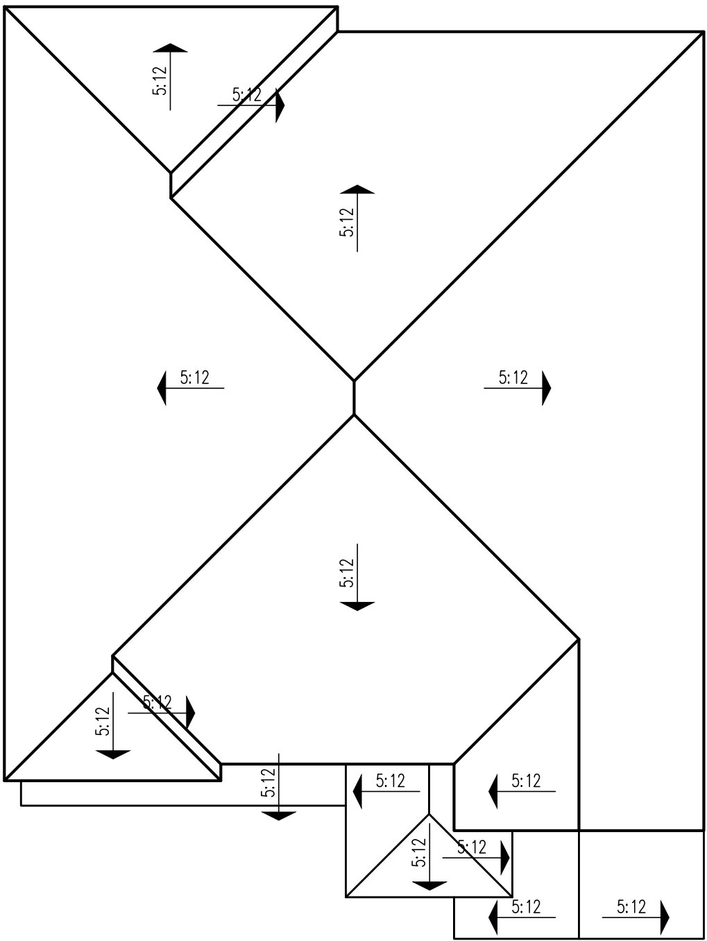
Roof Plan 'A' - Spanish Eclectic
