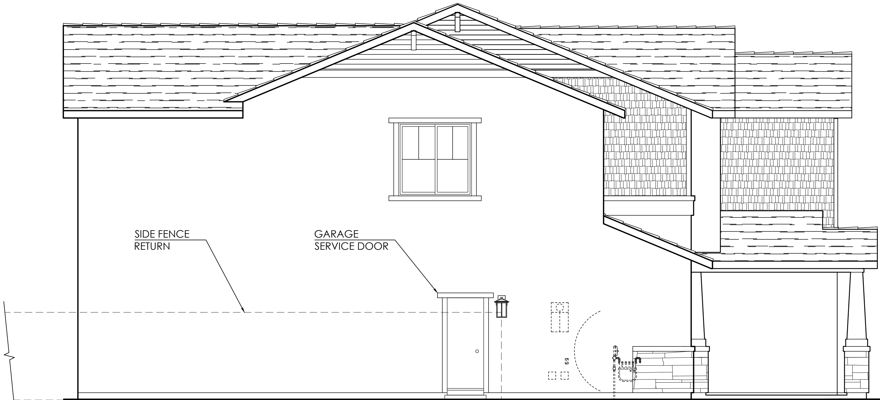
Left Elevation
