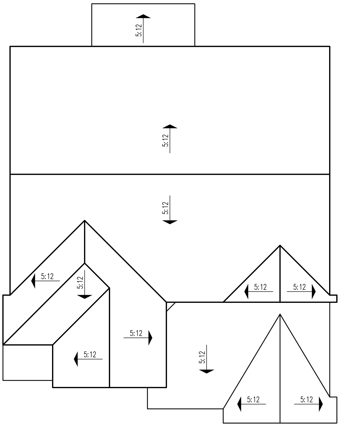
Roof Plan 'A' - Spanish Eclectic
