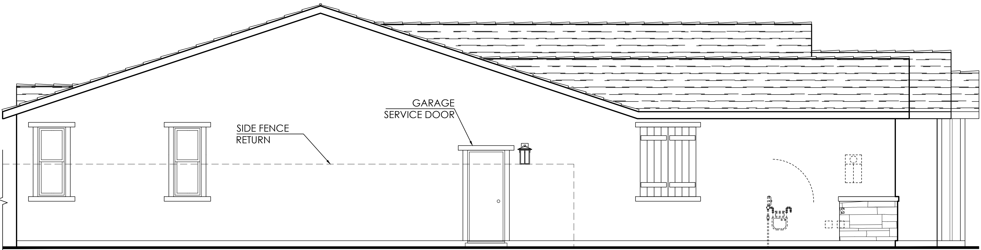
Left Elevation
