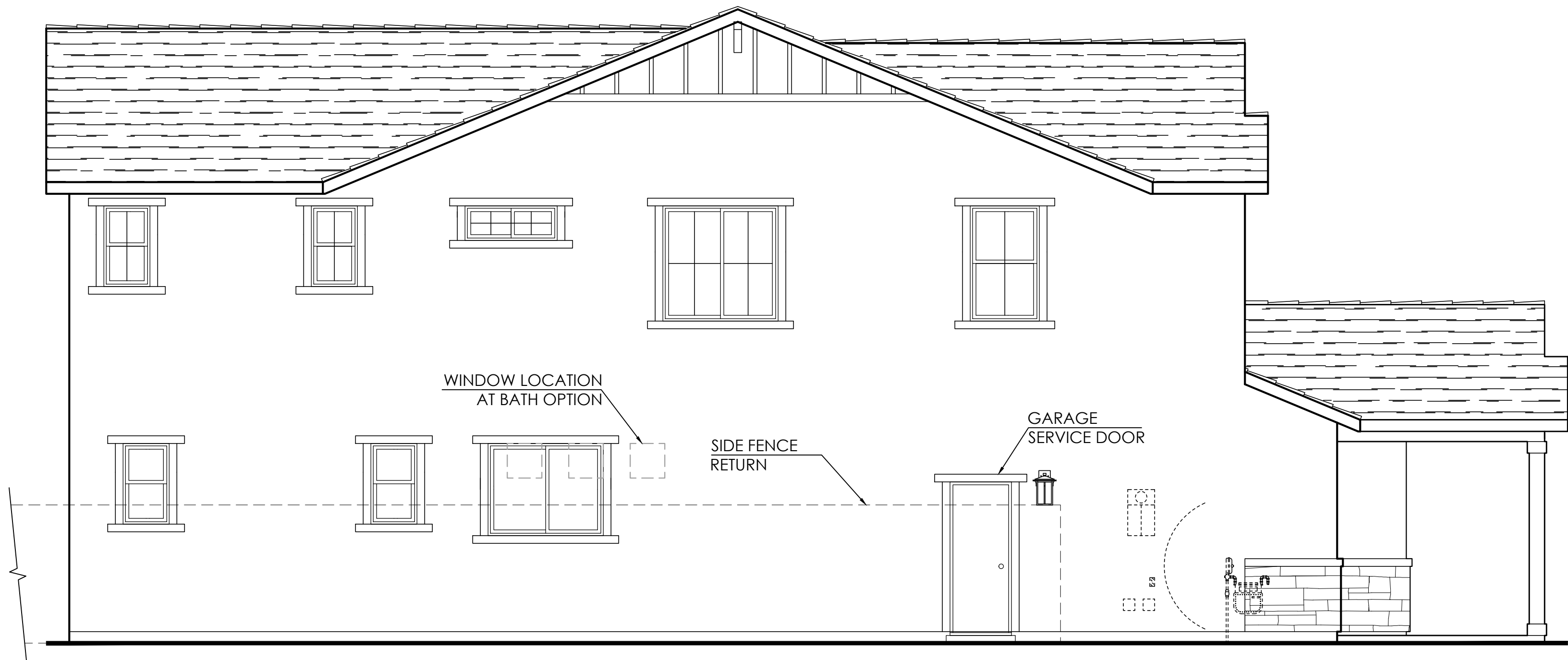
Left Elevation
