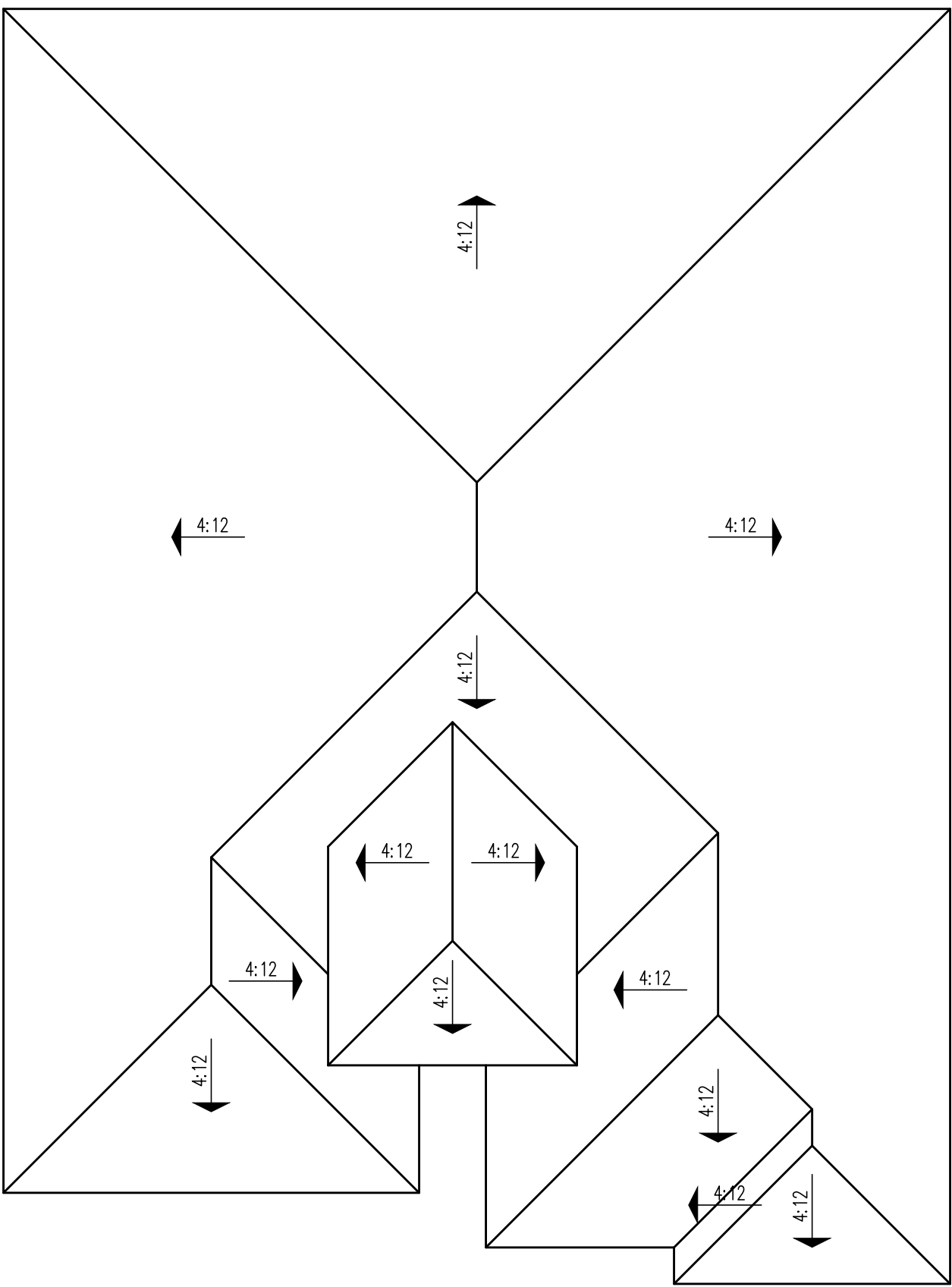
Roof Plan 'B' - Tuscan
