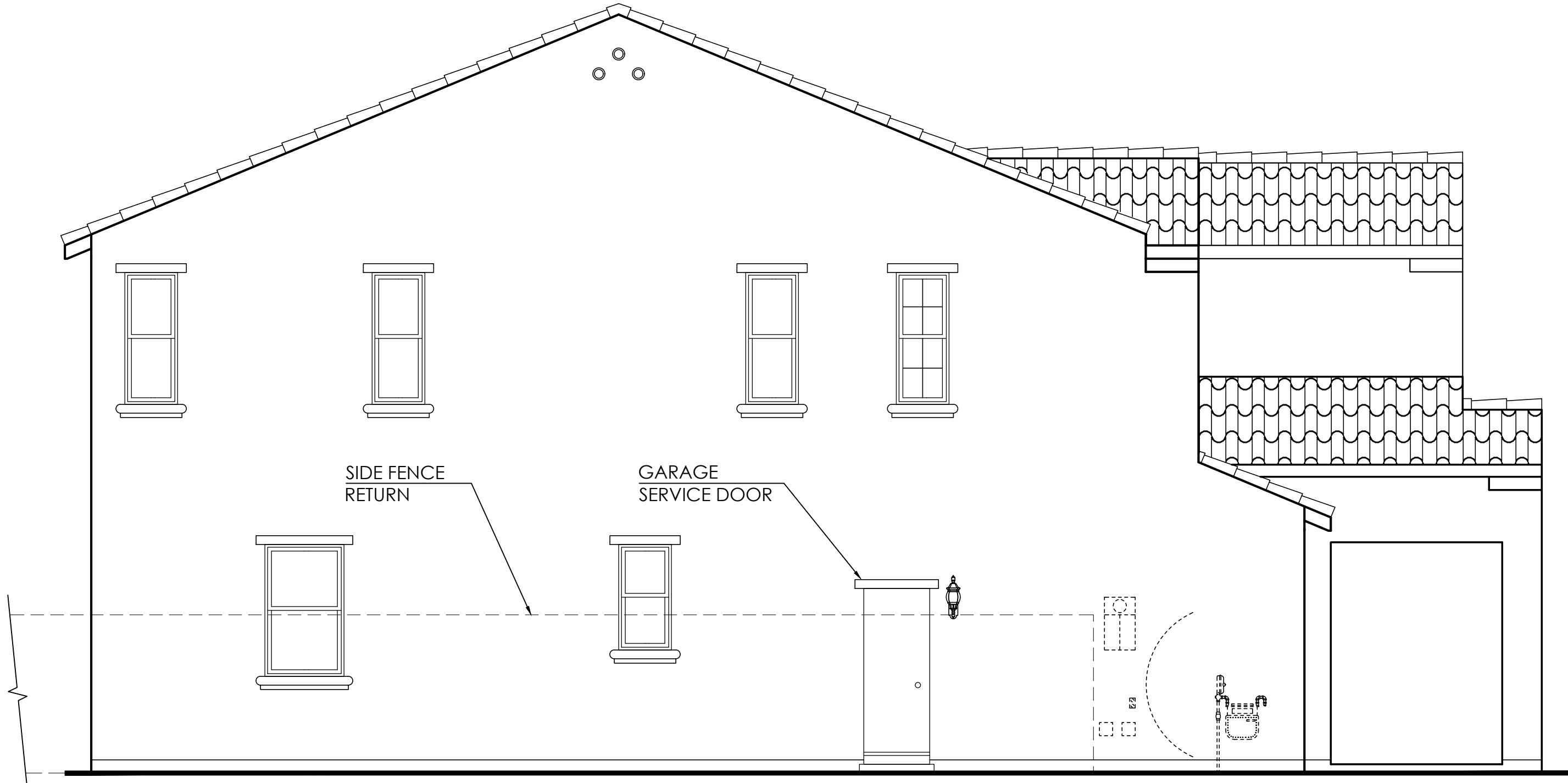
Left Elevation
