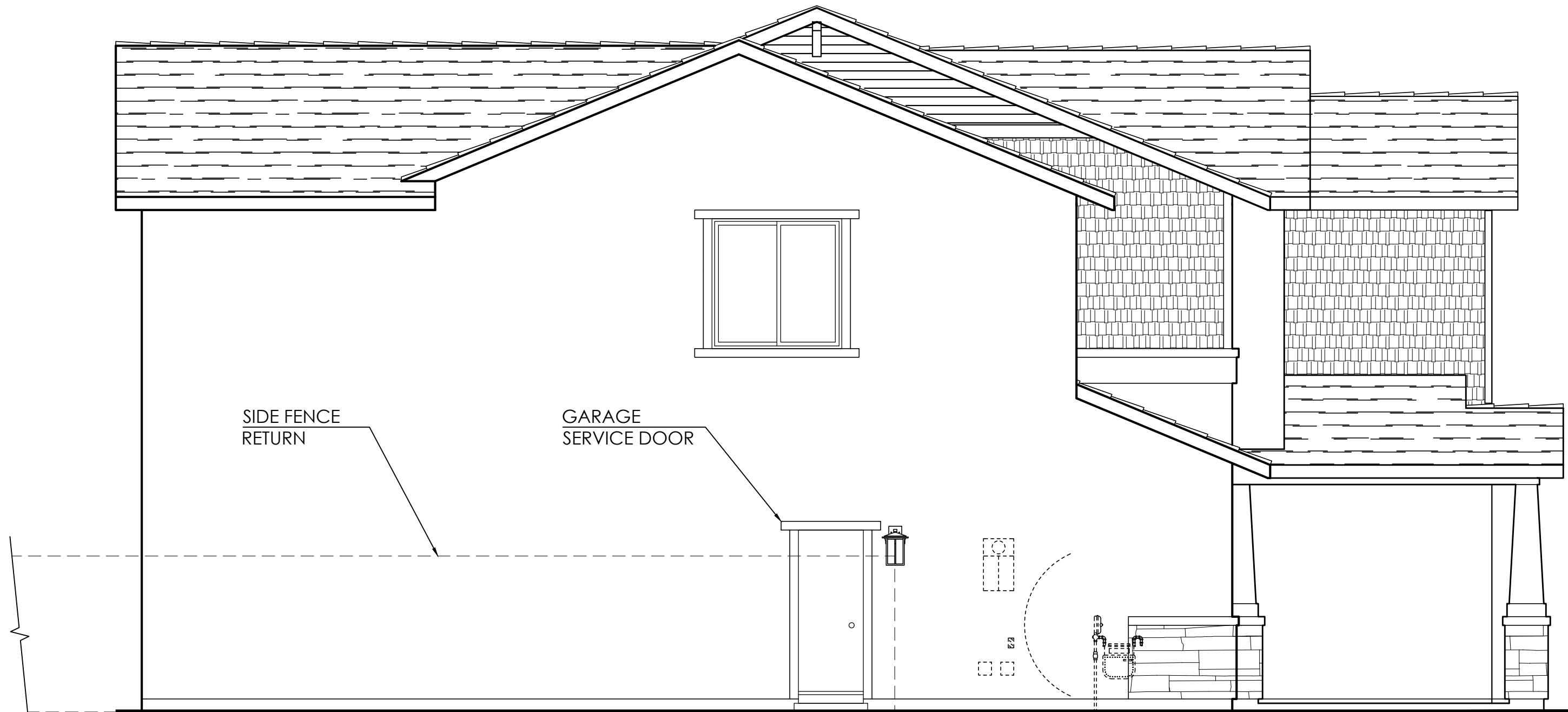
Left Elevation
