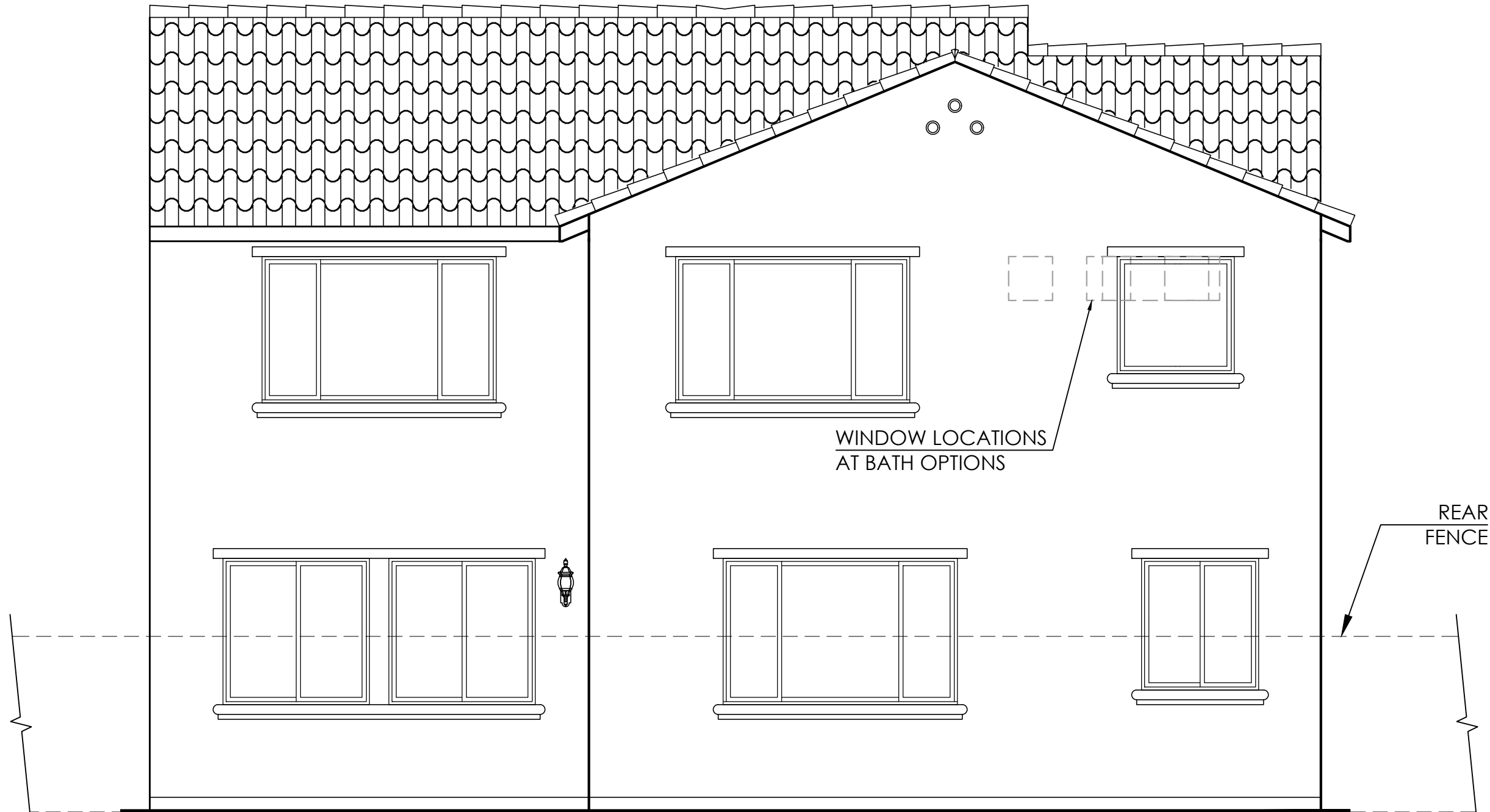
Rear Elevation
