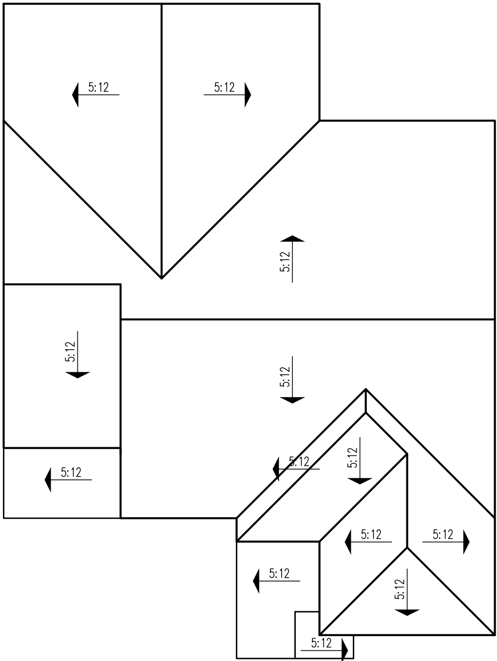
Roof Plan 'B' - California Tuscan
