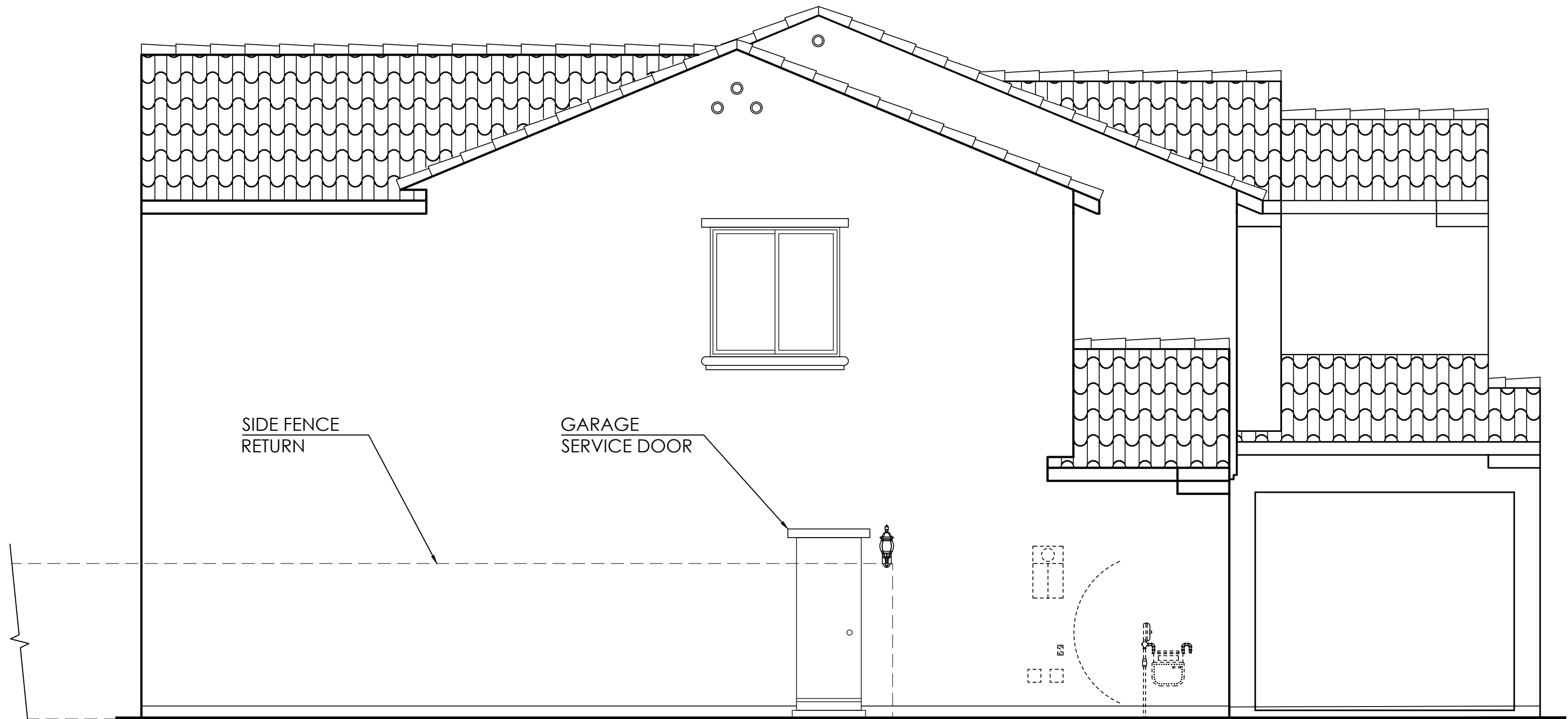
Left Elevation
