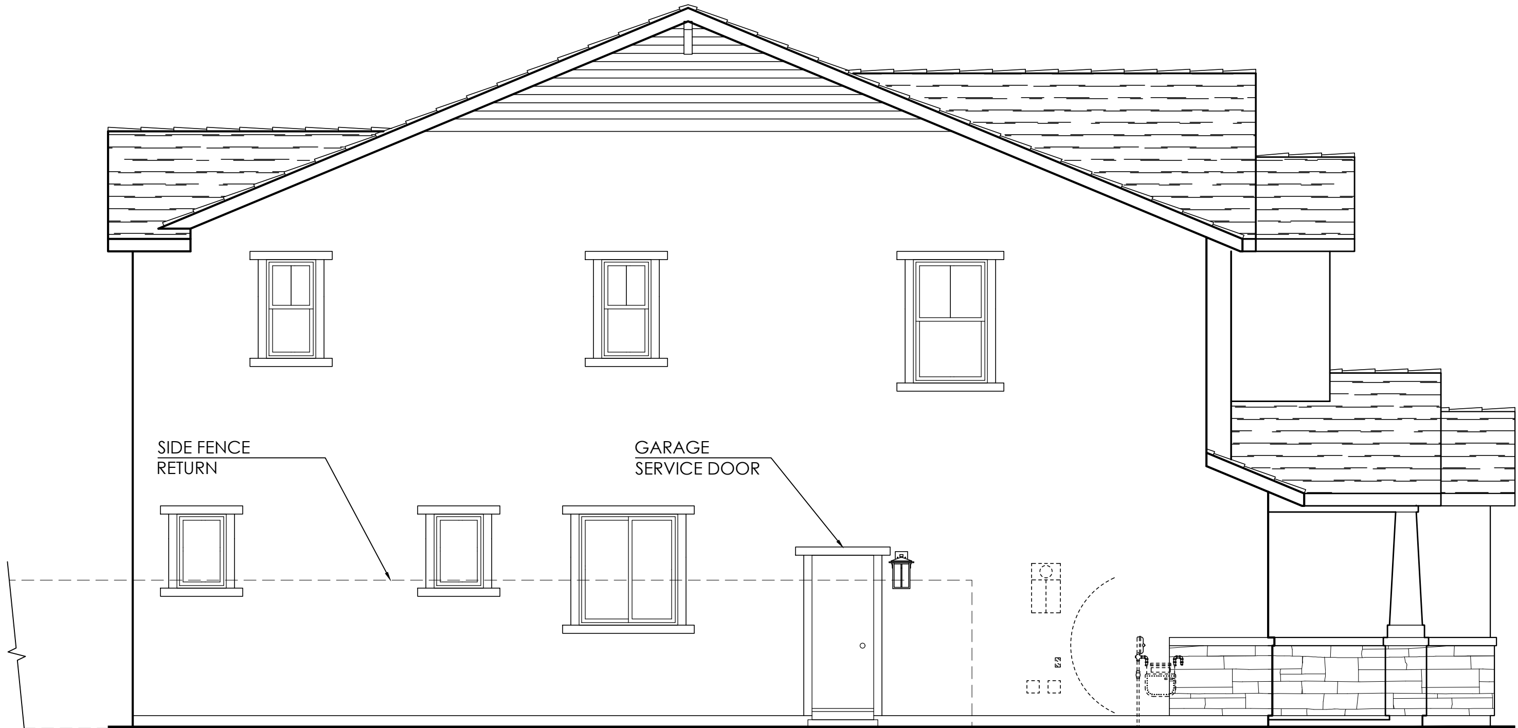
Left Elevation
