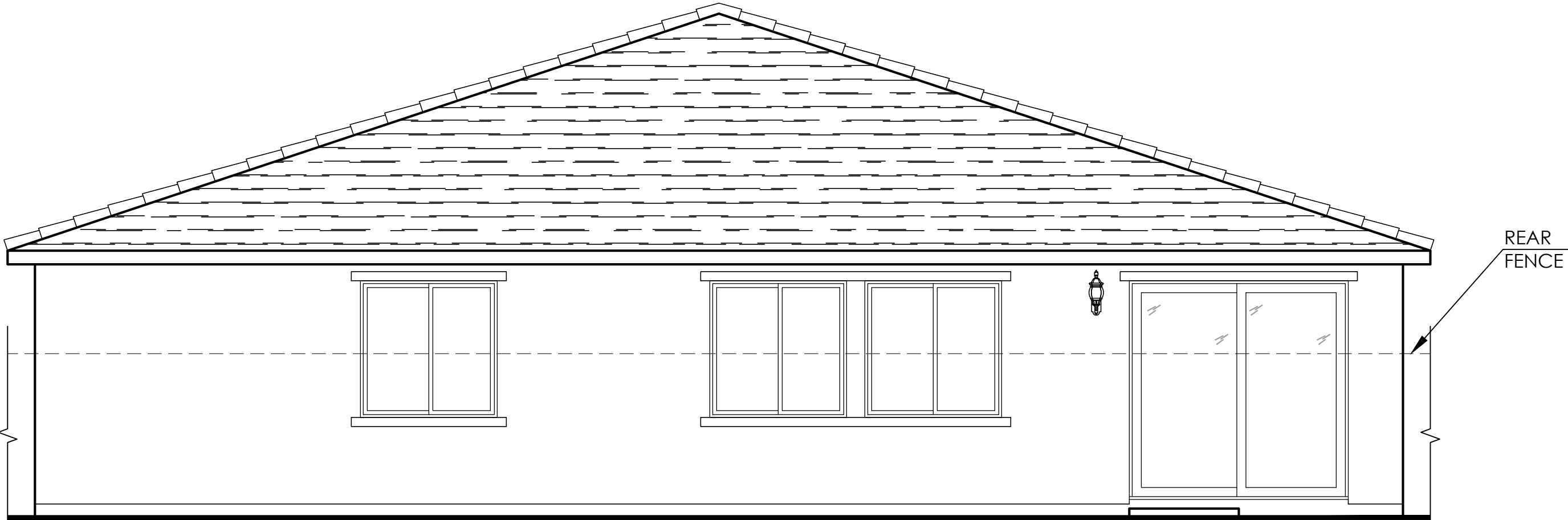
Rear Elevation
