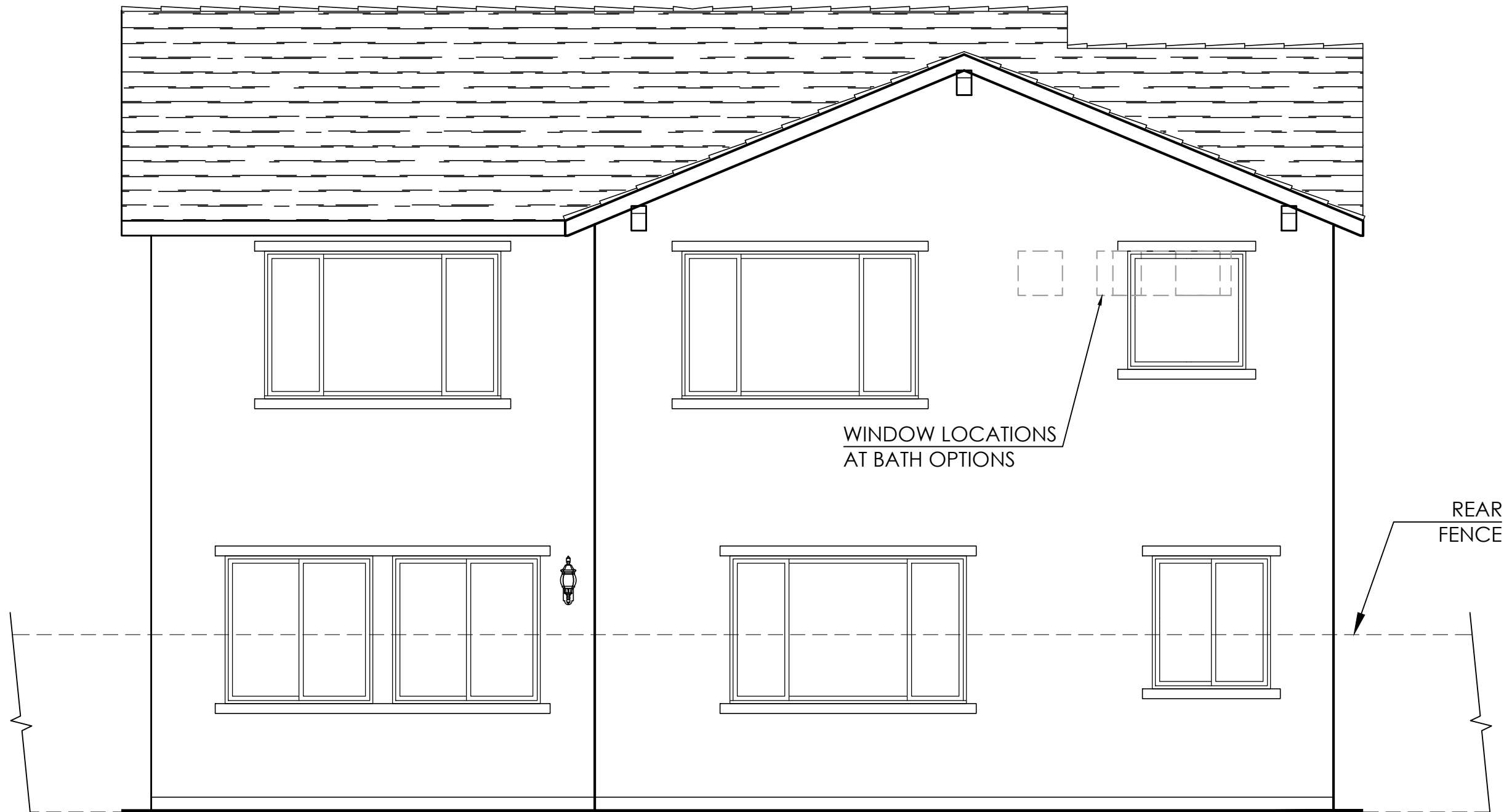
Rear Elevation
