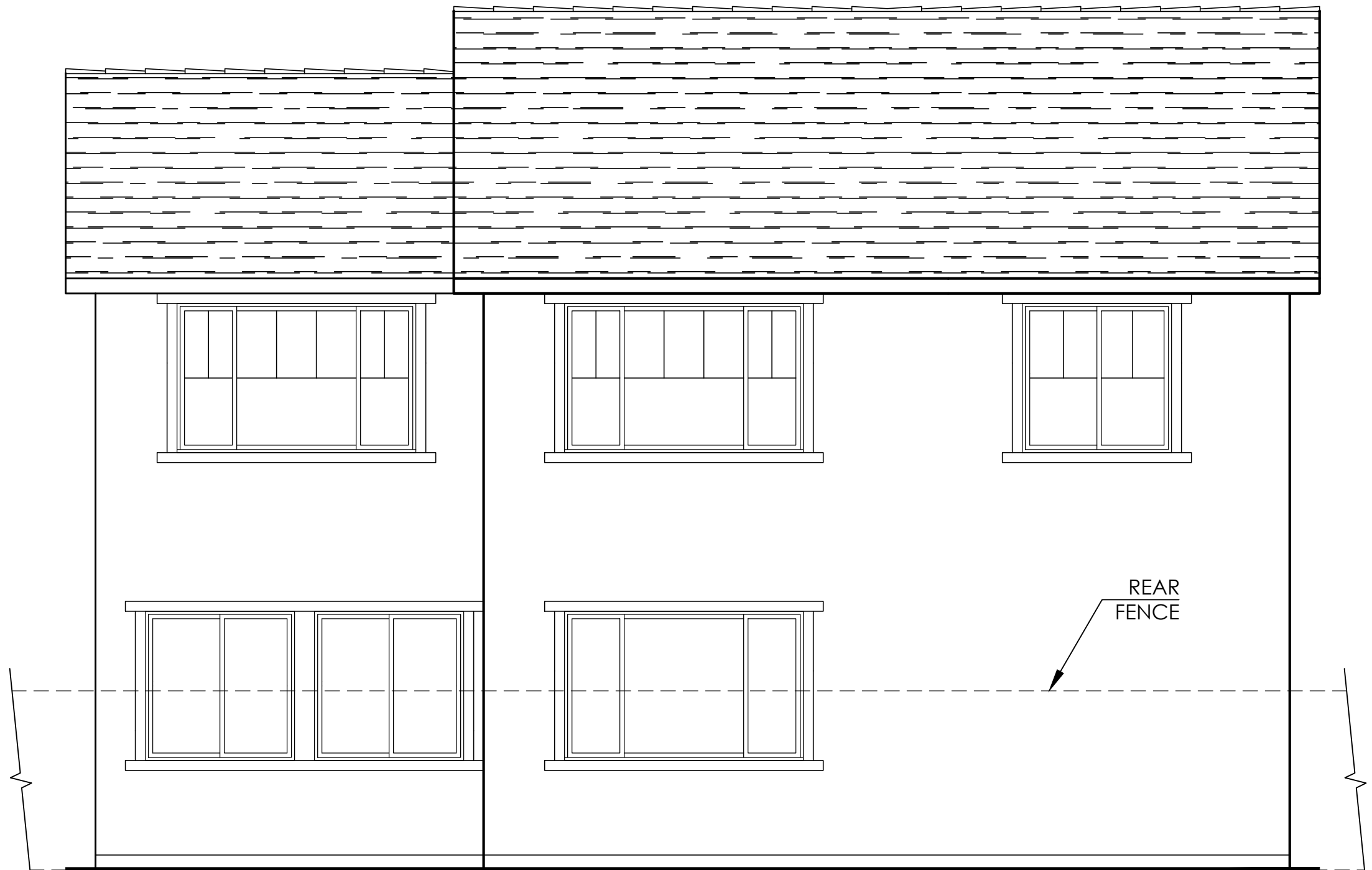
Rear Elevation
