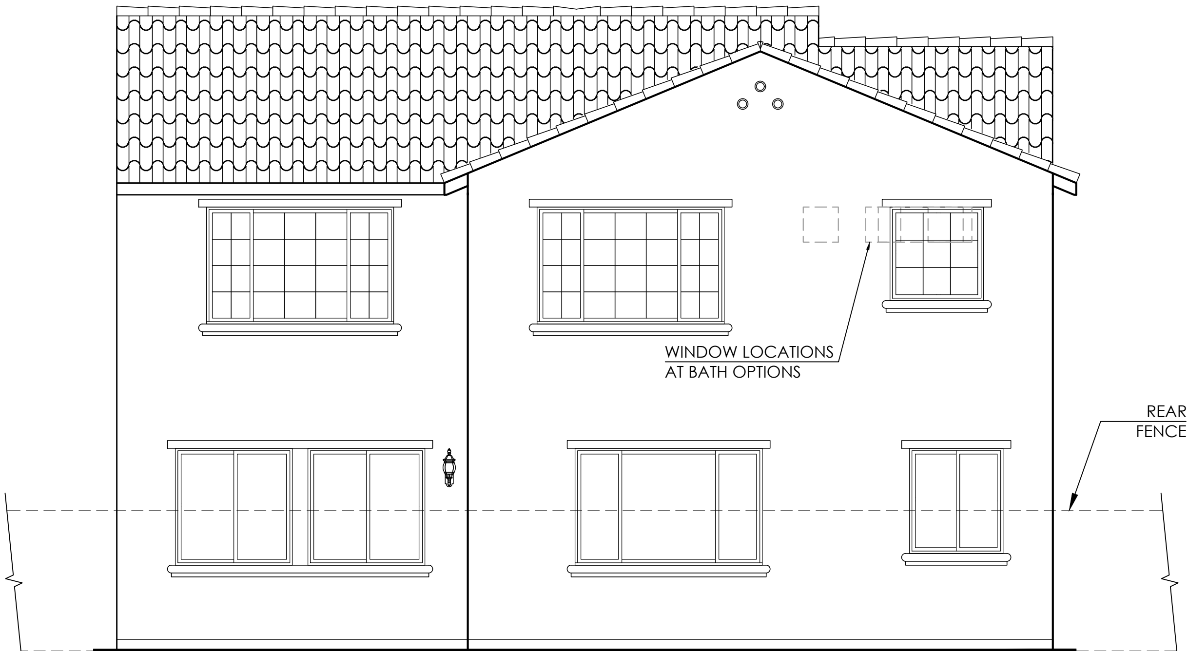
Rear Elevation
