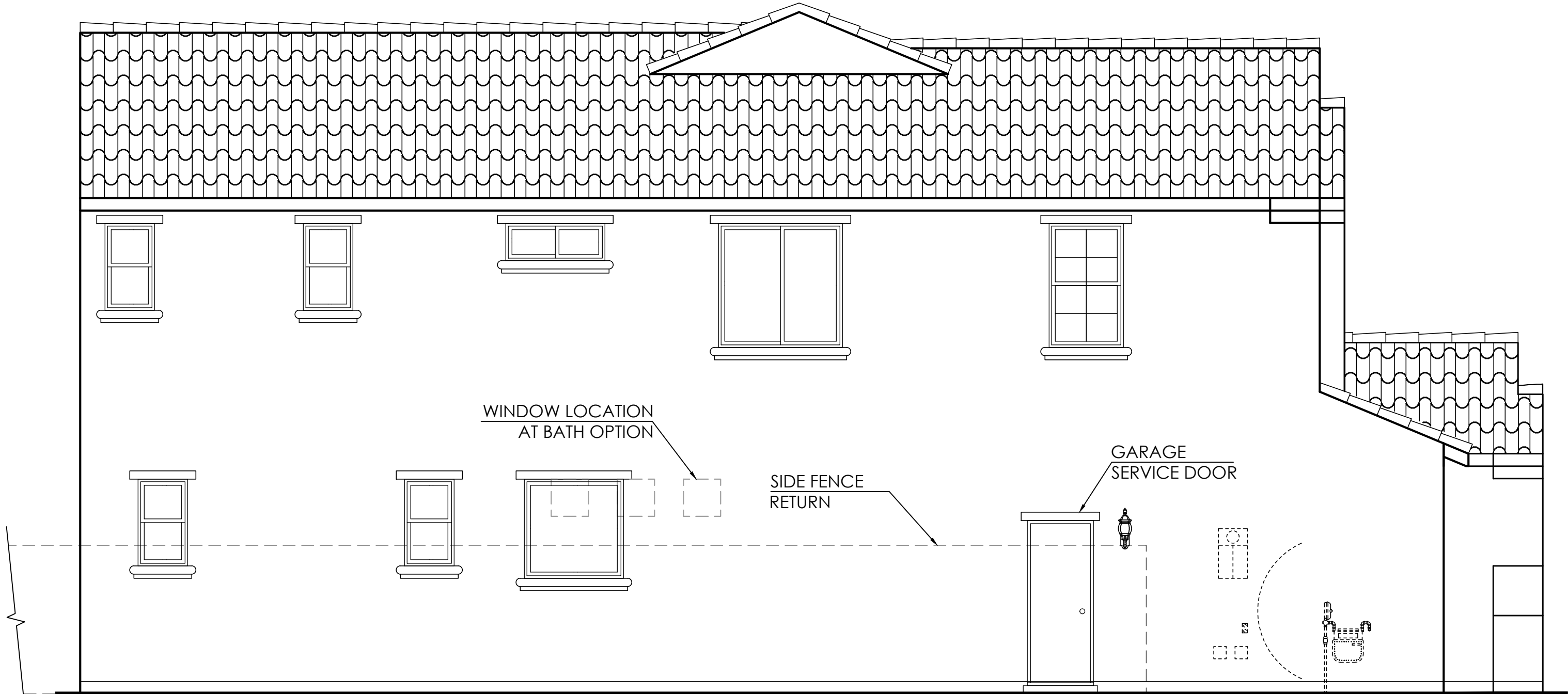
Left Elevation
