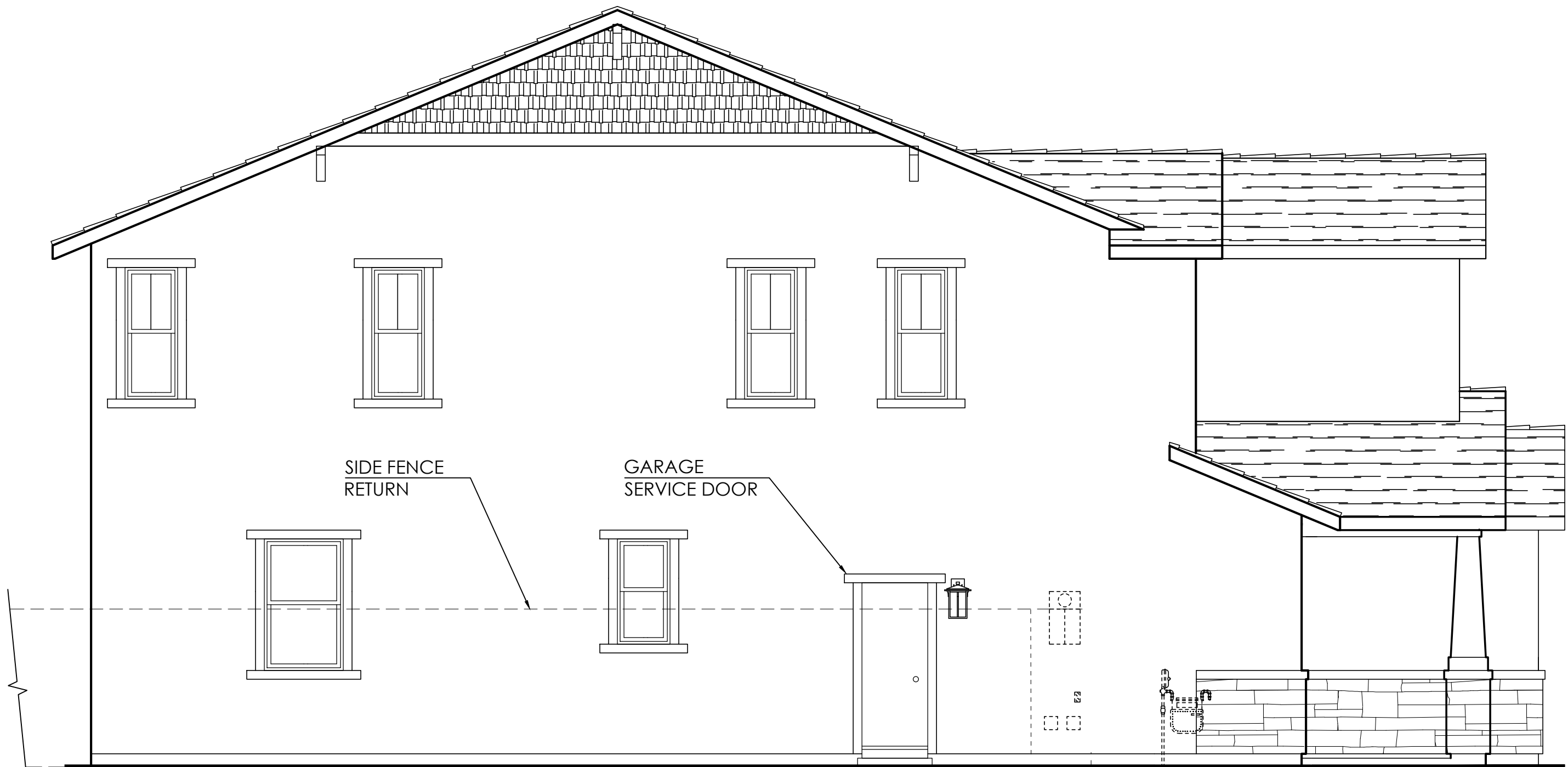
Left Elevation
