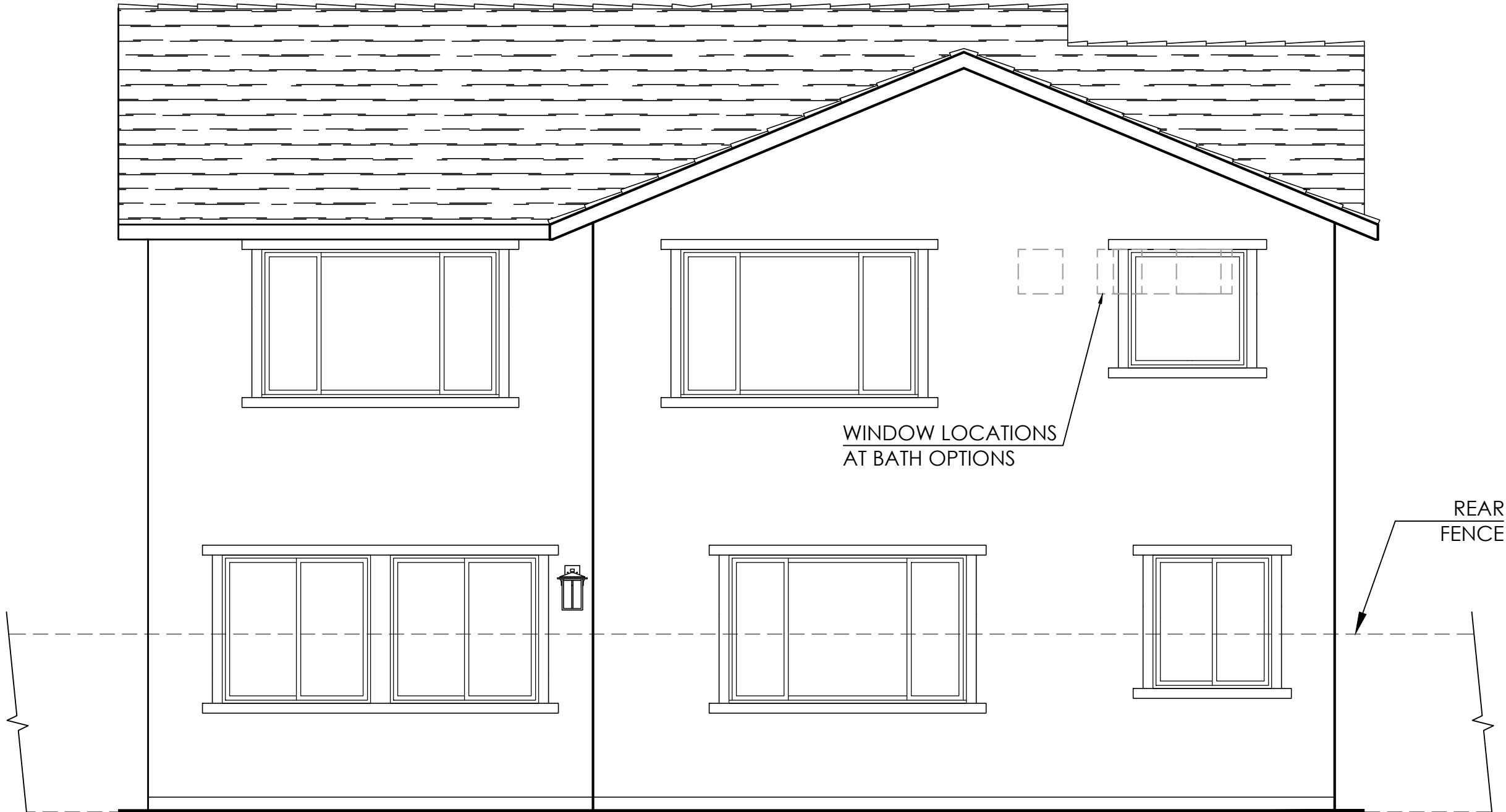
Rear Elevation
