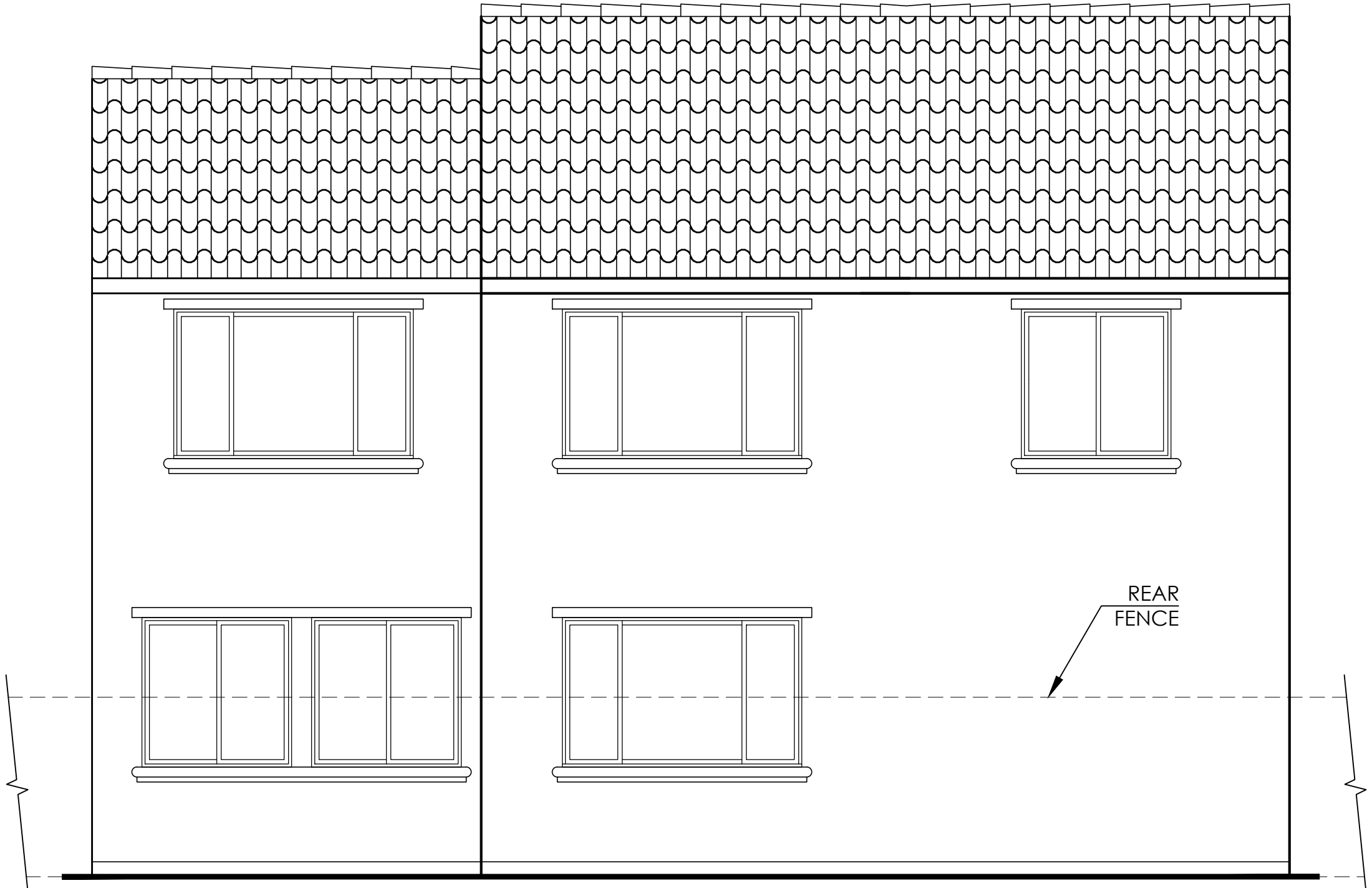
Rear Elevation
