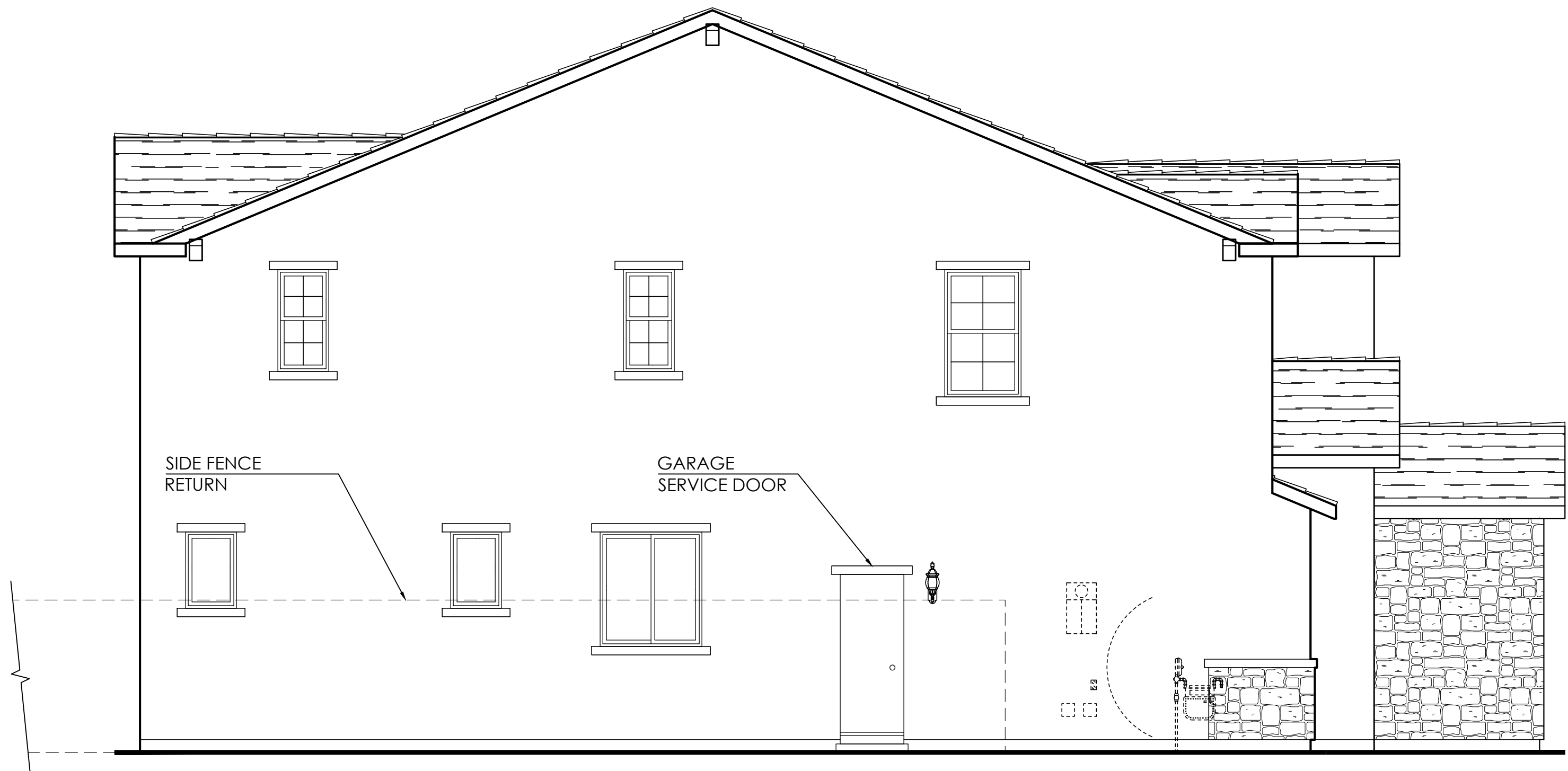
Left Elevation
