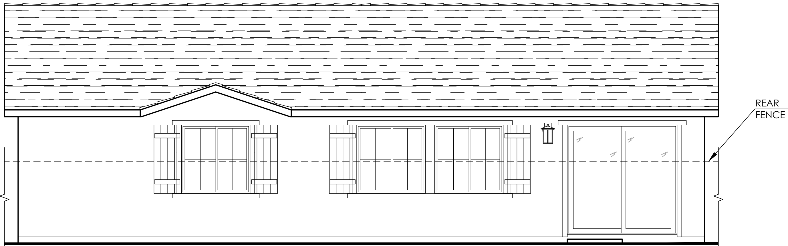
Rear Elevation
