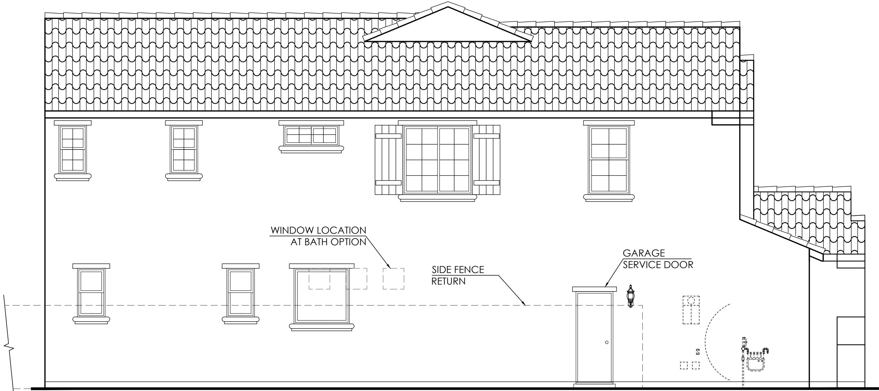
Left Elevation
