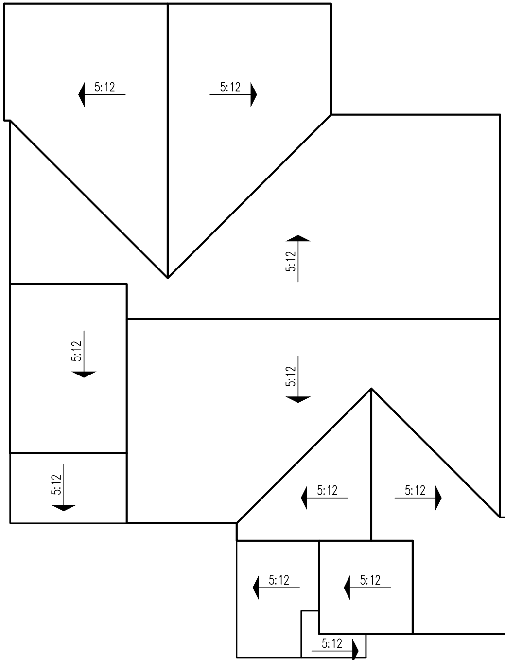
Roof Plan 'C' - Craftsman
