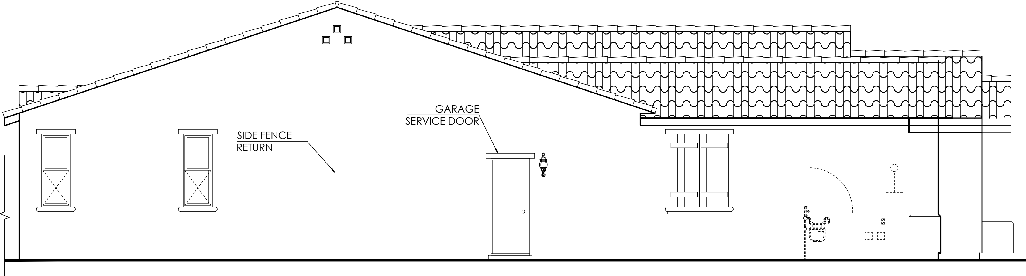
Left Elevation
