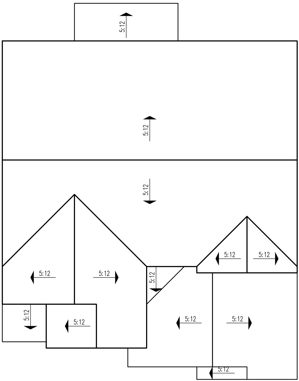
Roof Plan 'C' - Modern Farmhouse
