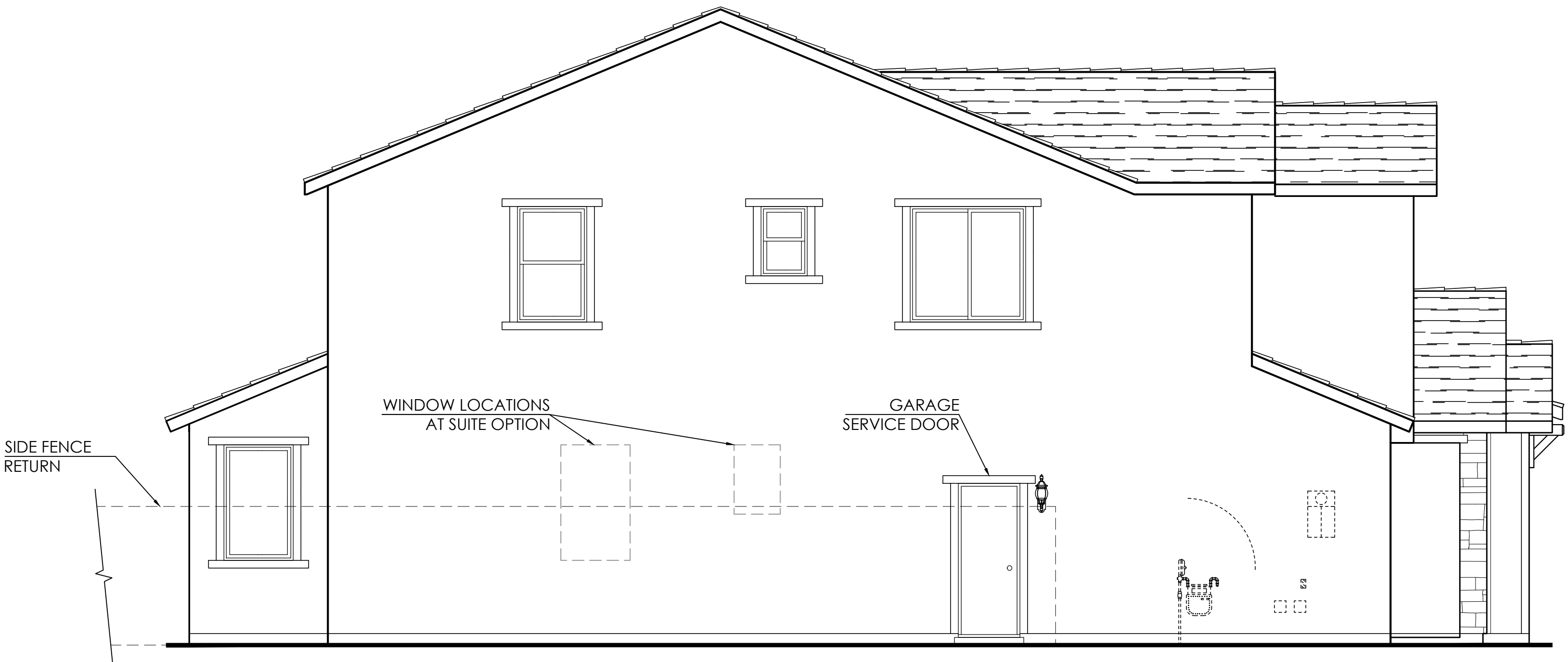
Left Elevation
