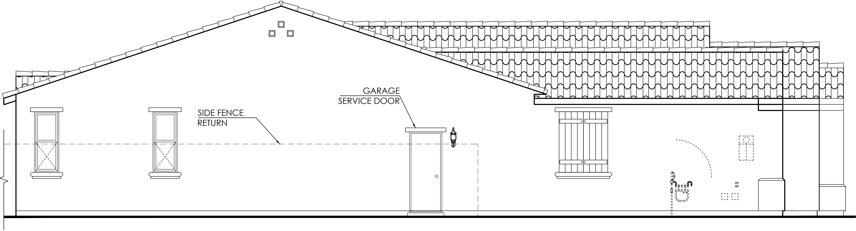
Left Elevation
