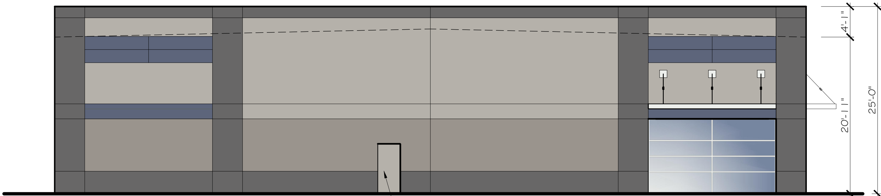
EAST ELEVATION
