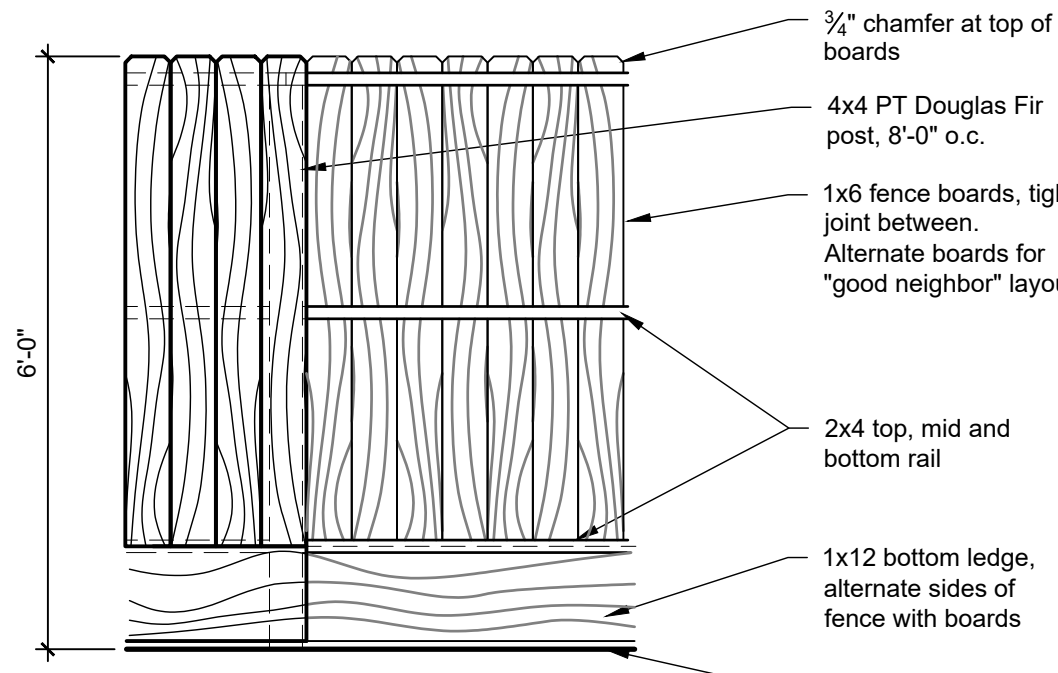
B Good Neighbor Fence
