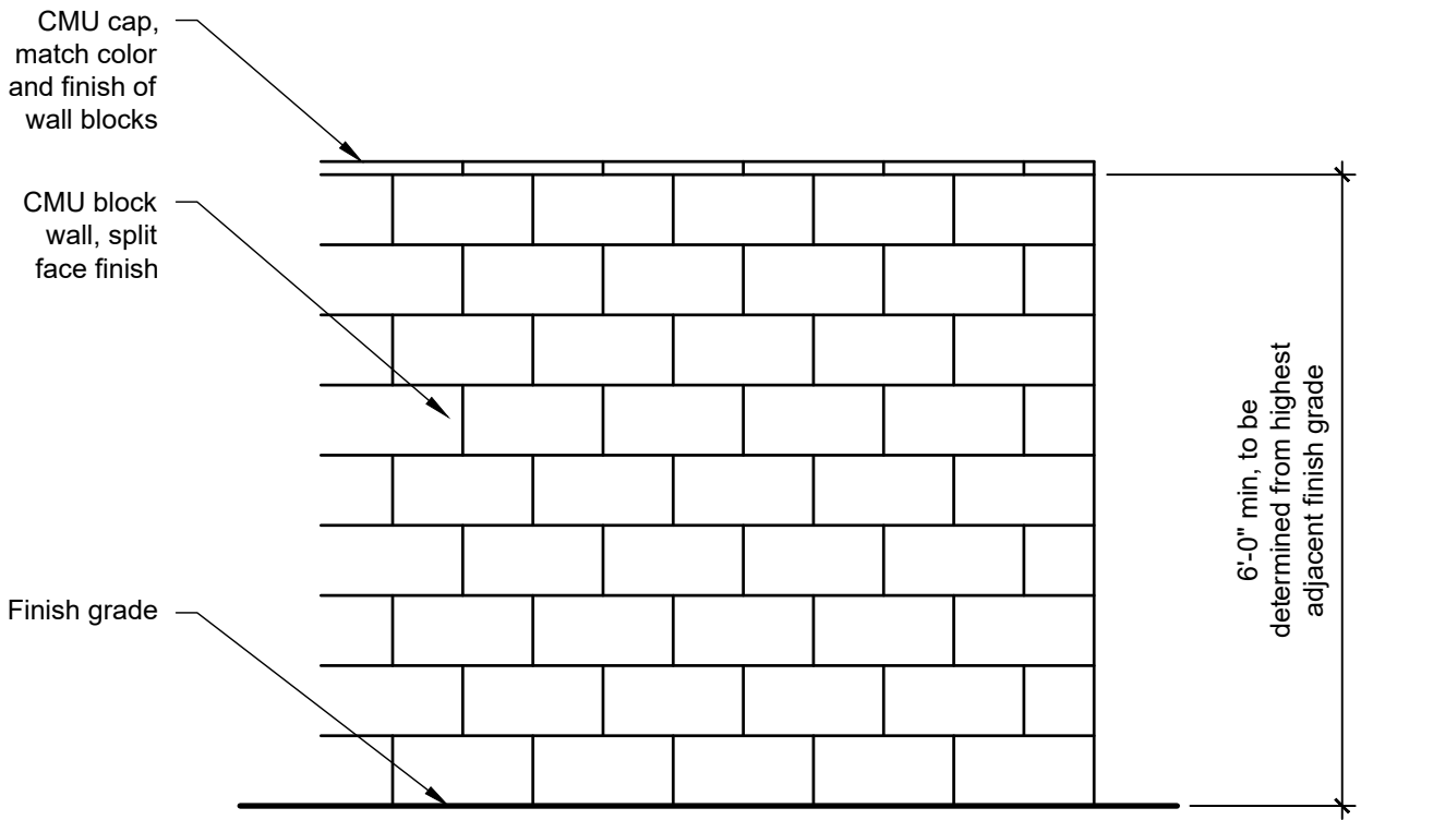
A CMU Perimeter Wall
