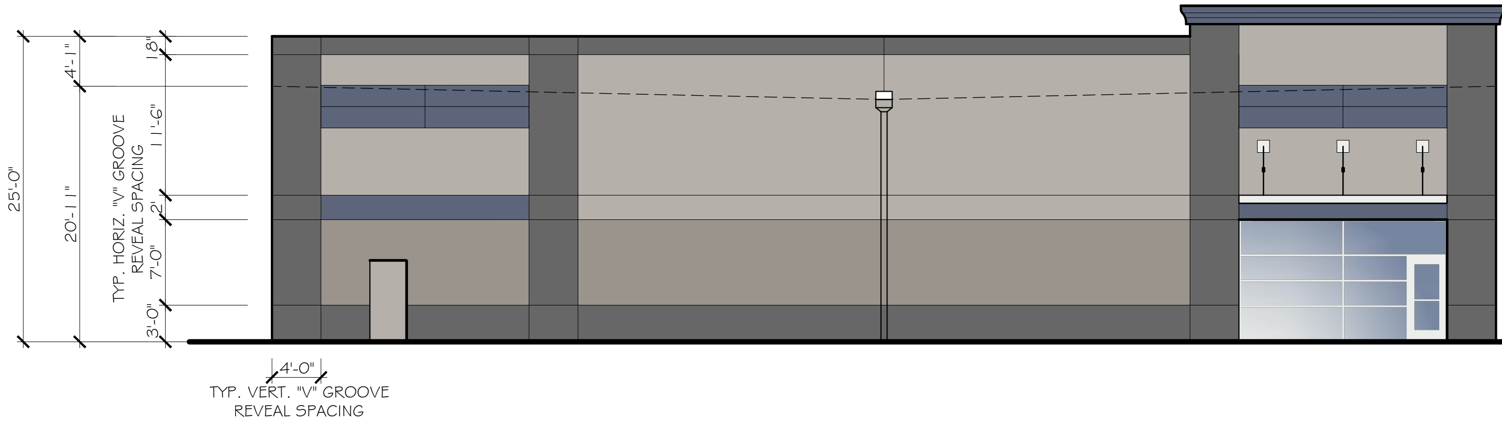
NORTH ELEVATION BUILDING 5 1/8" = 1'-0"
