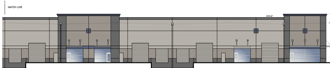
WEST ELEVATION
