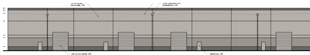
EAST ELEVATION
