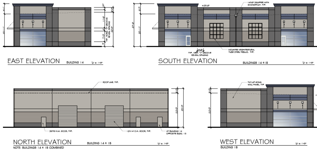
Figure 8: Building Perspectives
