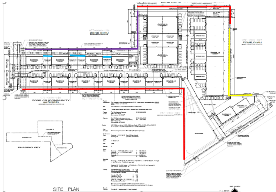
Figure 6: Proposed Fence/Wall Locations
