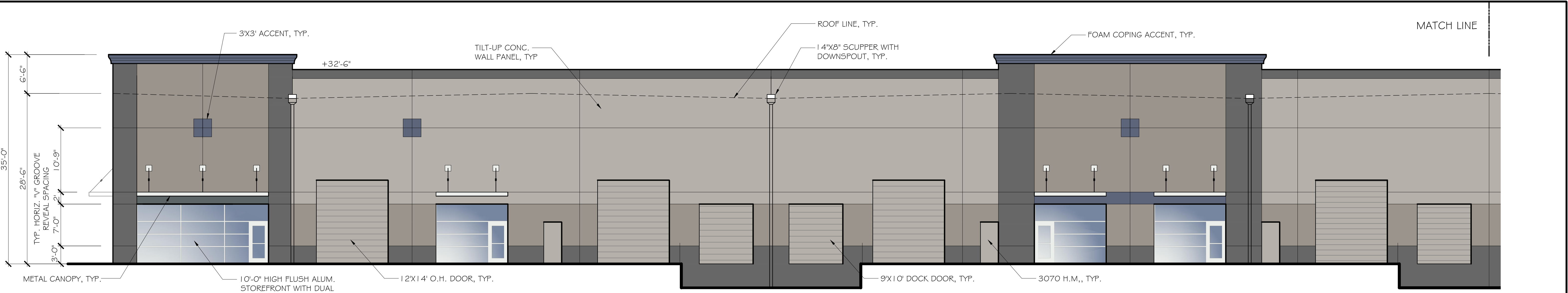
WEST ELEVATION
