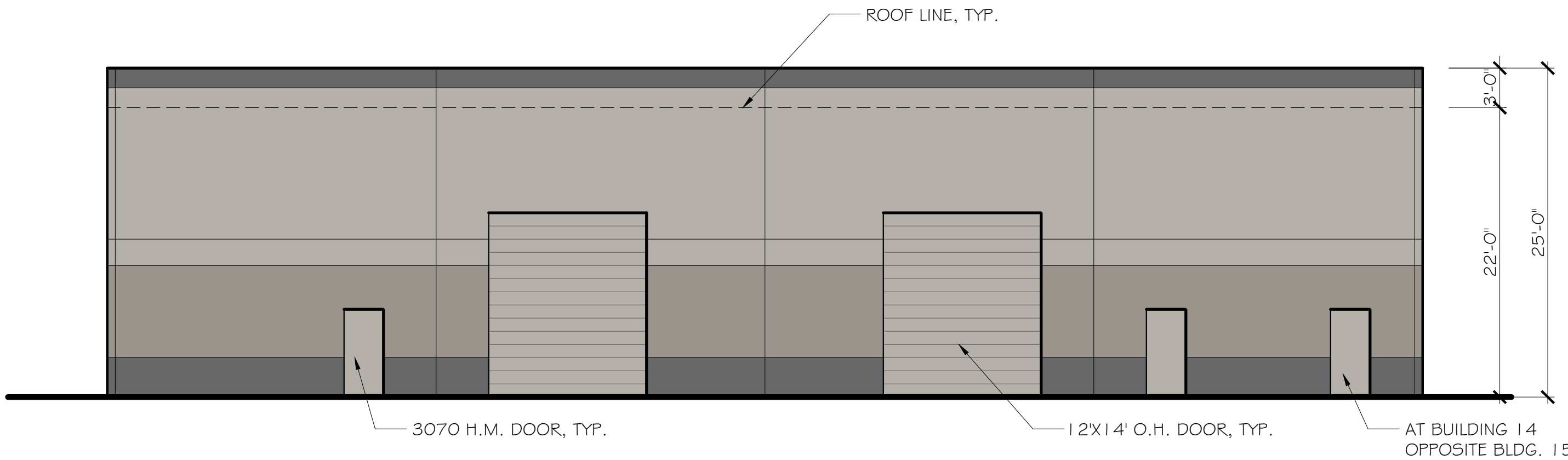
NORTH ELEVATION BUILDING 14 & 15 1/8" = 1'-0" NOTE: BUILDINGS 14 & 15 COMBINED
