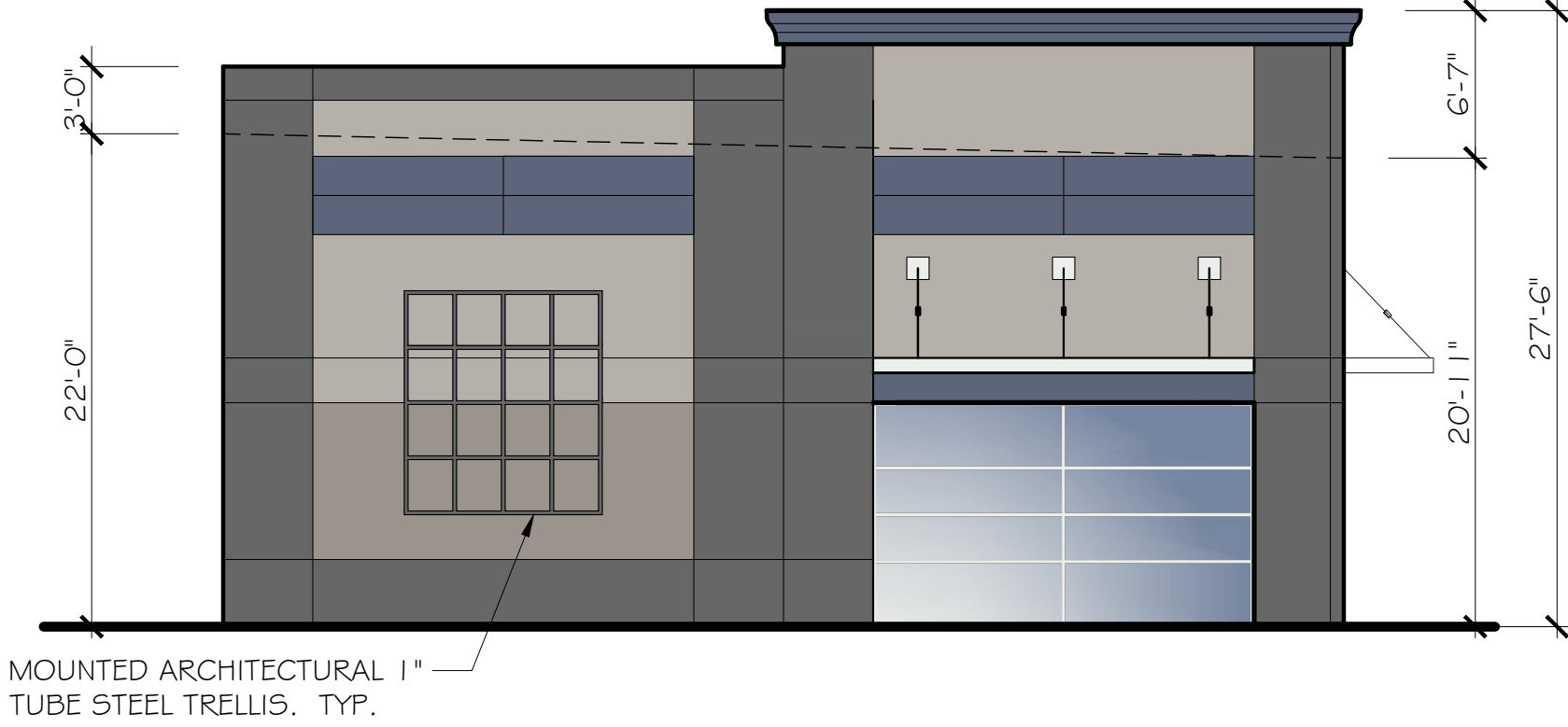
WEST ELEVATION BUILDING 1 1/8" = 1'-0"
