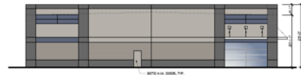
EAST ELEVATION BUILDINGS 11 & 12 1/8" = 1'-0"
