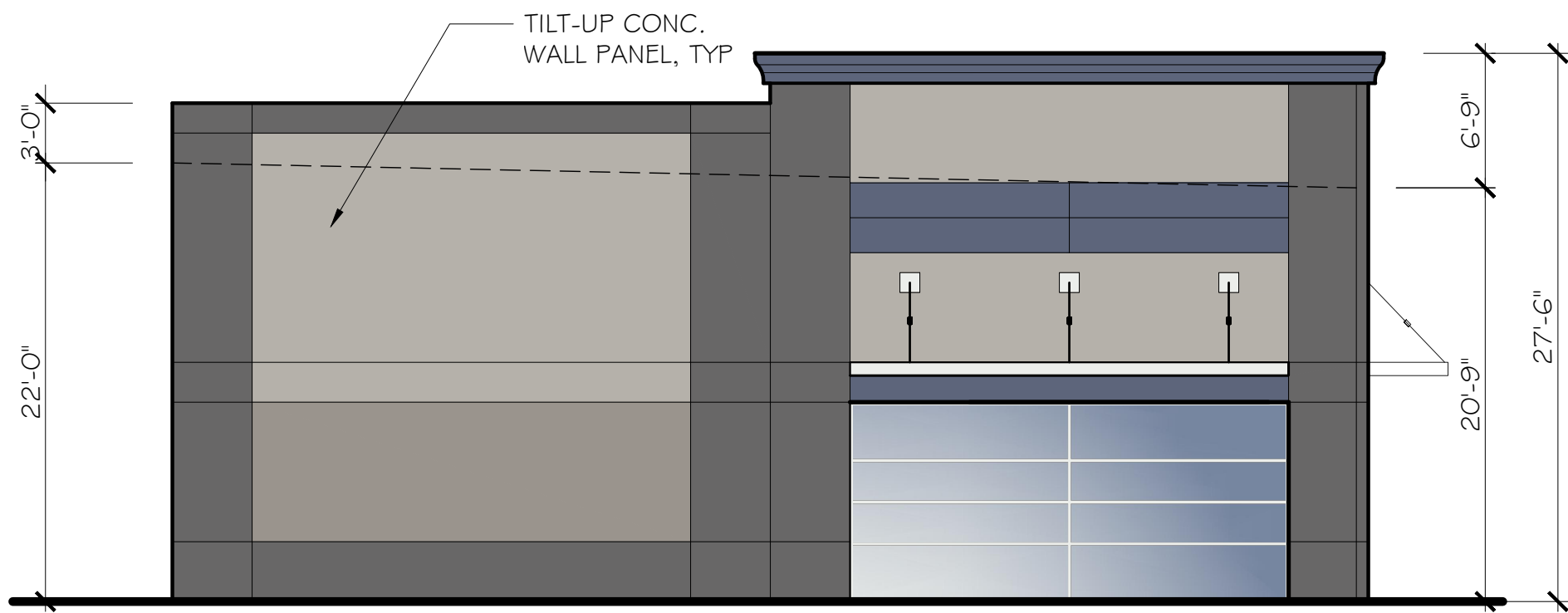
WEST ELEVATION BUILDING 15 1/8" = 1'-0"
