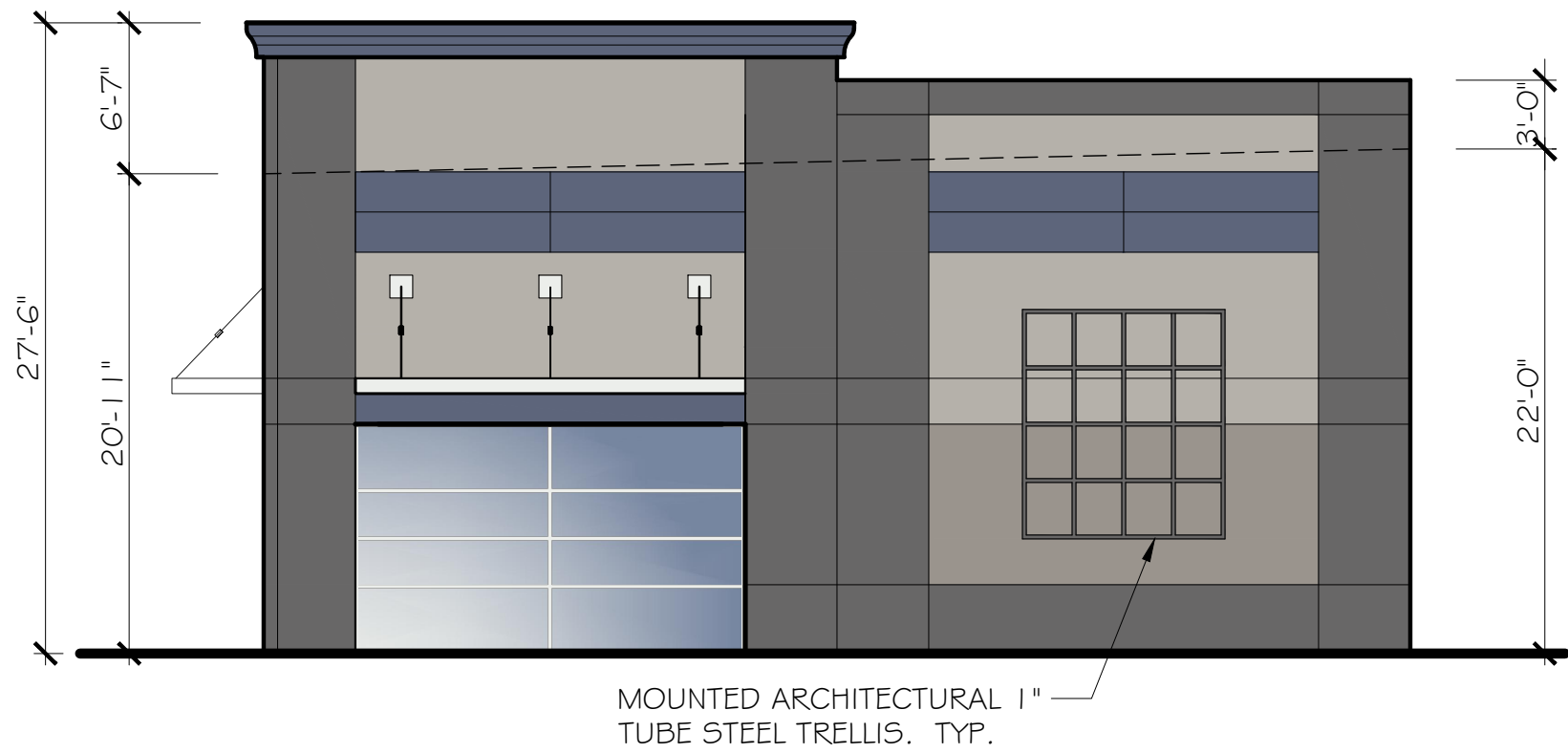
WEST ELEVATION BUILDING 5 1/8" = 1'-0"
