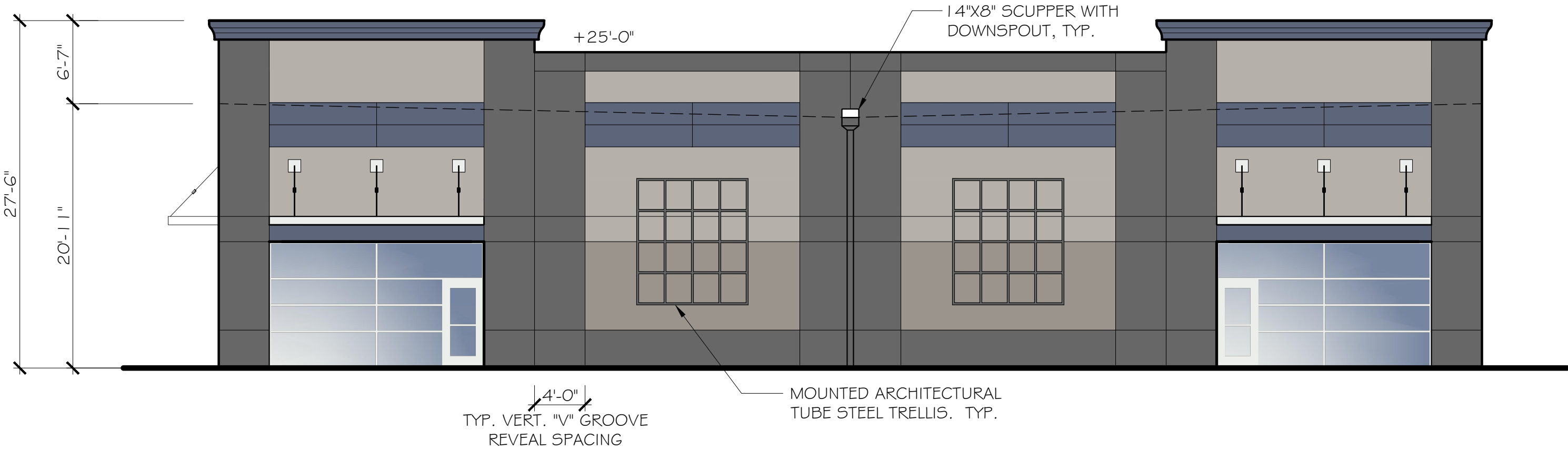
SOUTH ELEVATION BUILDINGS 14 & 15 1/8" = 1'-0"
