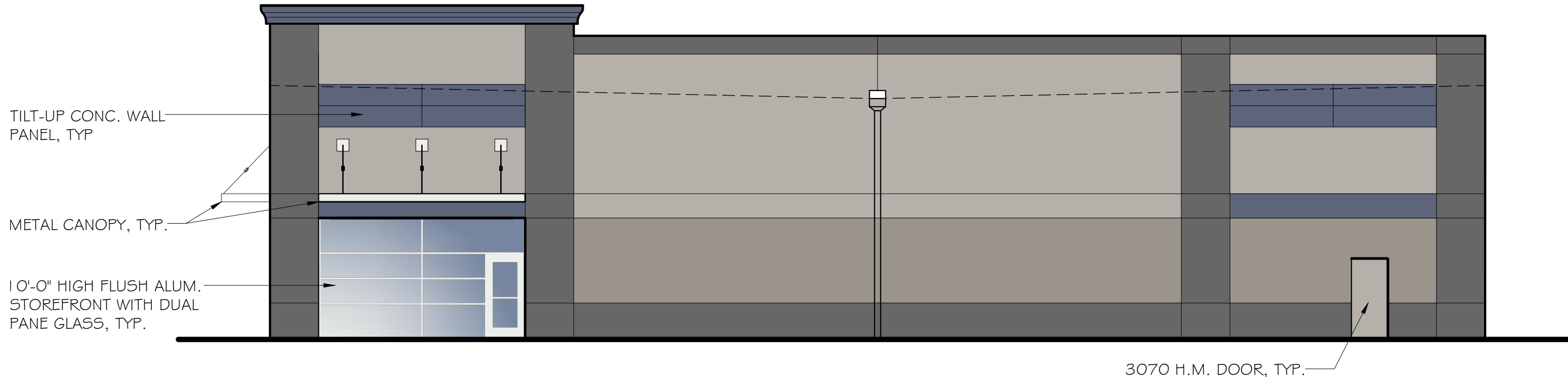
SOUTH ELEVATION BUILDING 1 1/8" = 1'-0"
