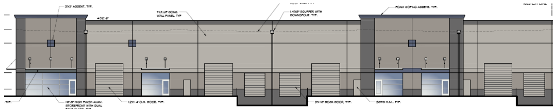
WEST ELEVATION
