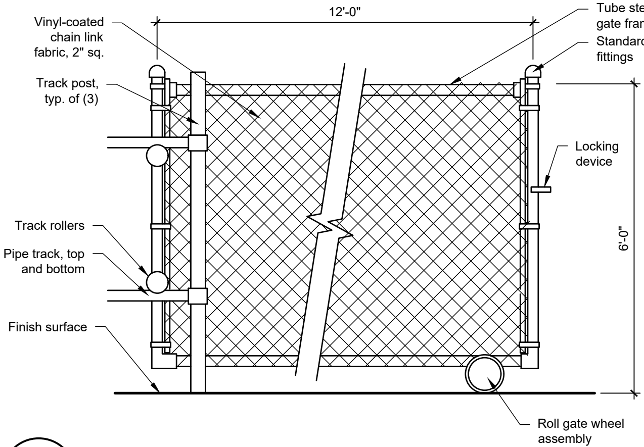
C Chain Link Rolling Gate
