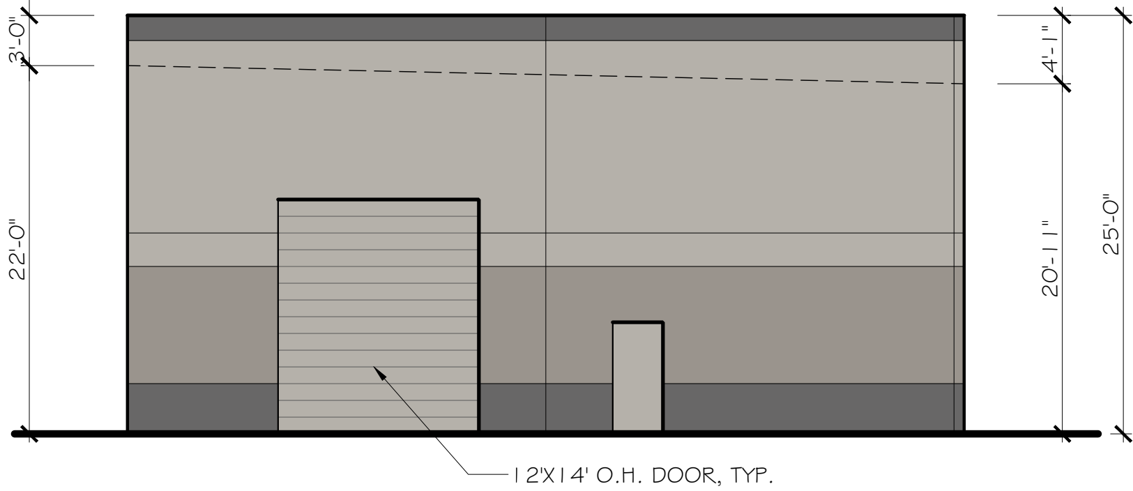
WEST ELEVATION BUILDINGS 3 & 4 1/8" = 1'-0" EAST ELEVATION BUILDINGS 5-9
